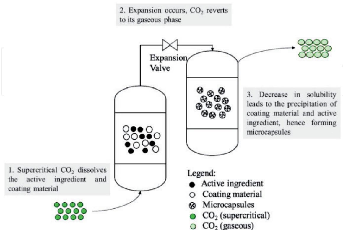
Figure 9. Schematic representation of the RESS process [86].
