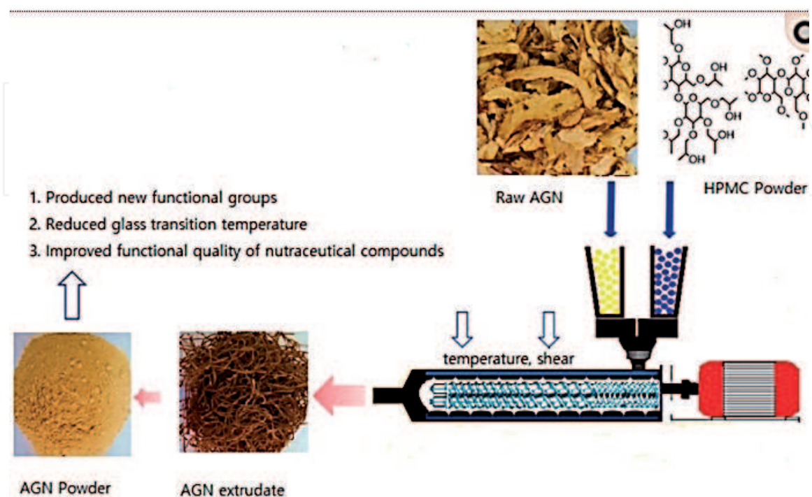
Figure 3. A schematic diagram of the hot melt extrusion process used in the encapsulation of Angelica gigas Nakai (AGN) [38].
