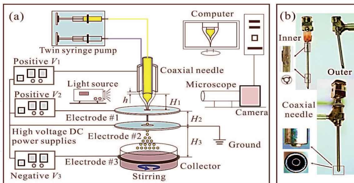
Figure 7. (a) Coaxial assembly for electrospaying. (b) Inner and outer coaxial needles [59].
