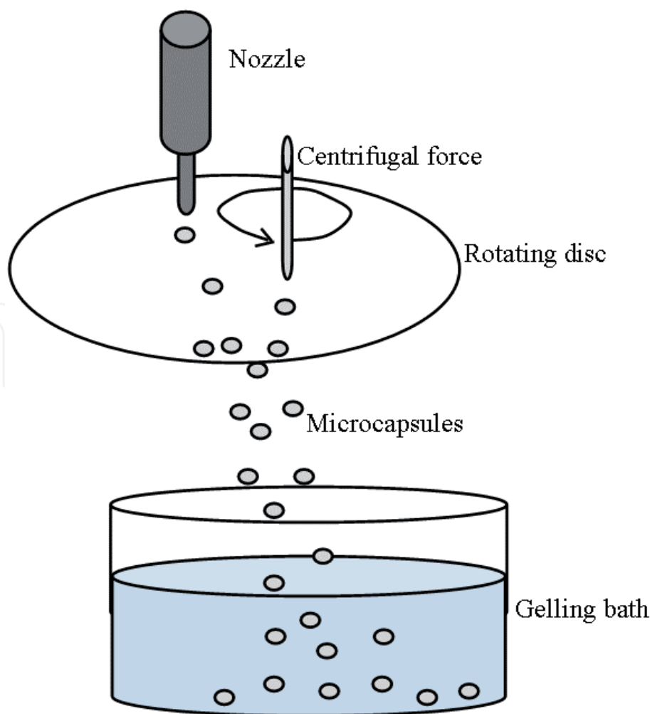
Figure 6. Schematic representation of the spinning disc assembly.
