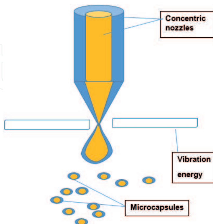
Figure 4. Schematic representation of the co-extrusion technique.
