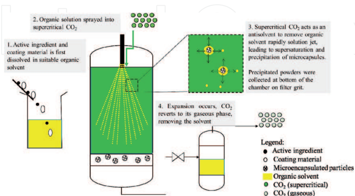
Figure 10. Schematic representation of the GAS process [86].
