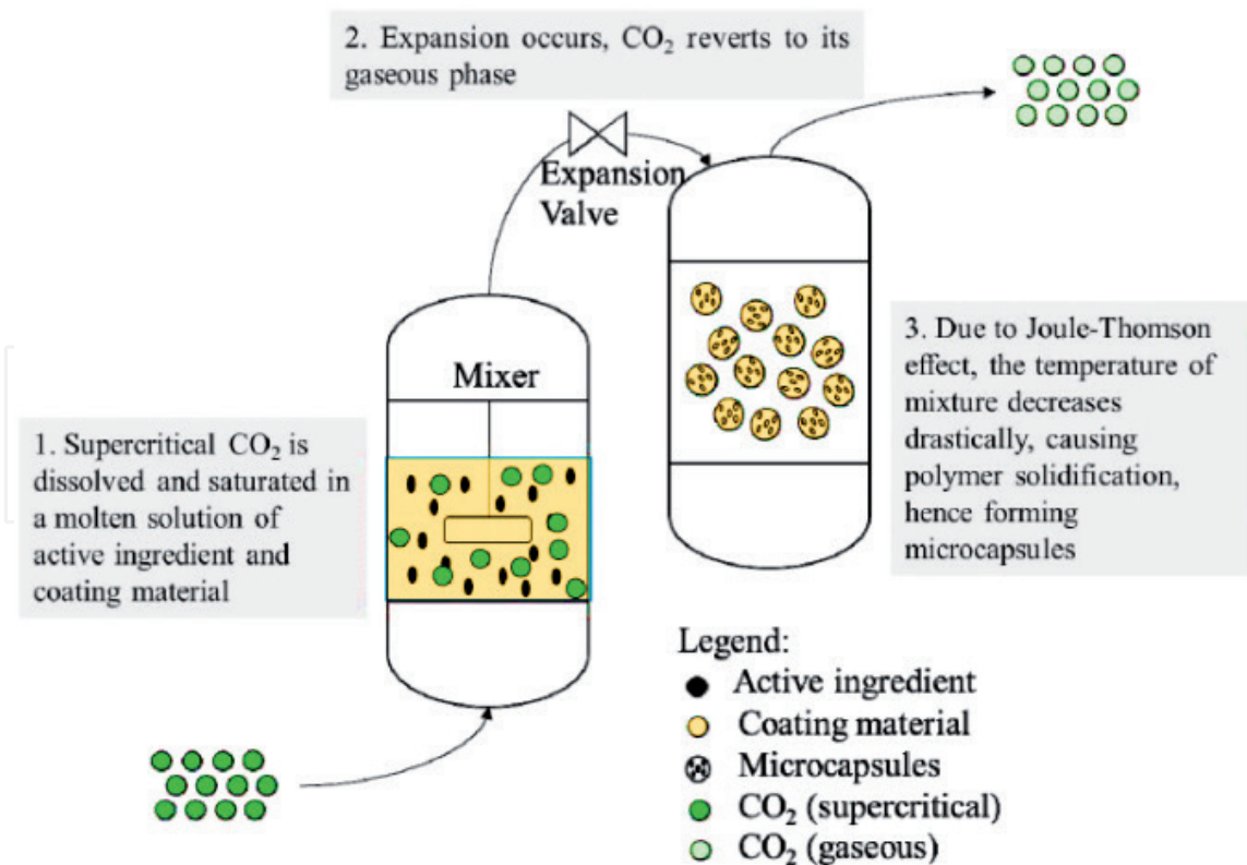
Figure 11. Schematic representation of the PGSS approach [86].
