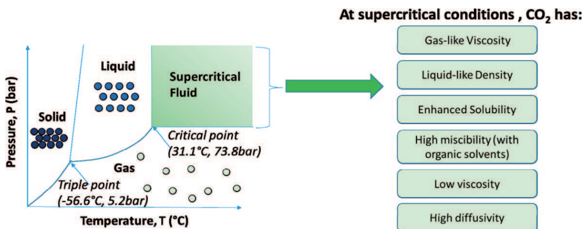
Figure 8. Phase diagram of SCCO 2 (not to scale) [86].
