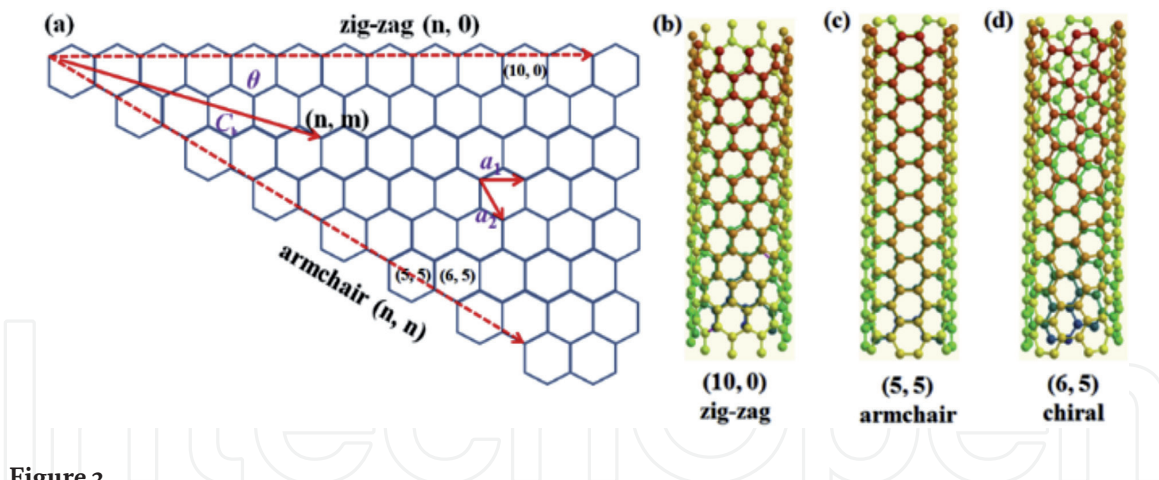
Figure 2. (a) Unrolled single-layer graphene sheet showing the geometry of the SWCNT, (b-d) Examples of the three types of nanotube sidewall; zigzag, armchair, and chiral (A color version of this figure can be viewed online) [42].
