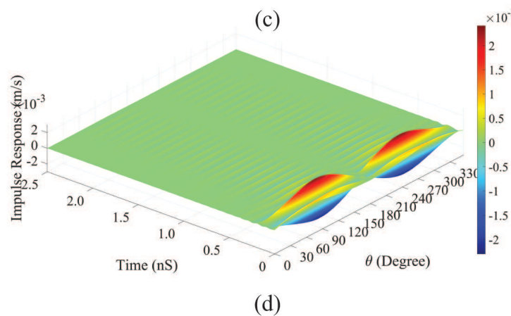
Figure 8. Computed transfer functions of the RMA in the (a) x-y (b) x-z planes; computed impulse responses the RMA in the (c) x-y (d) x-z planes.
