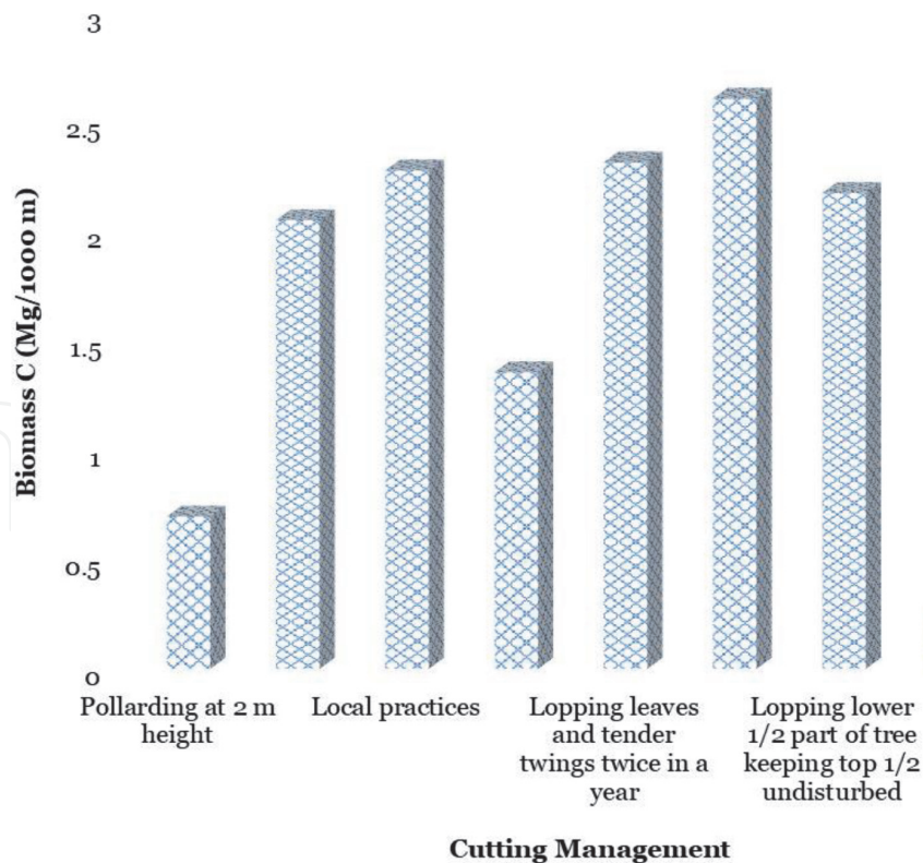
Figure 5. Biomass C stock in wayside plantation with different cutting management in Kachnar in wayside plantation.
