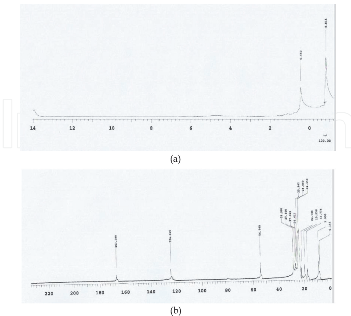
Figure 3. (a) ^1\text{H} NMR spectrum of the biodiesel. (b) ^{13}\text{C} NMR spectrum of the biodiesel.
