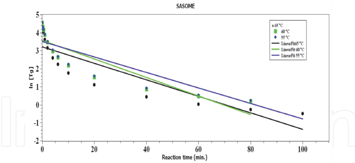
Figure 10. First-order plot of the triglycerides hydrolysis.
