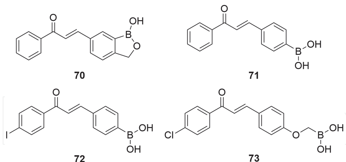
Figure 19. Chemical structures of boron-containing chalcones [76–80].
