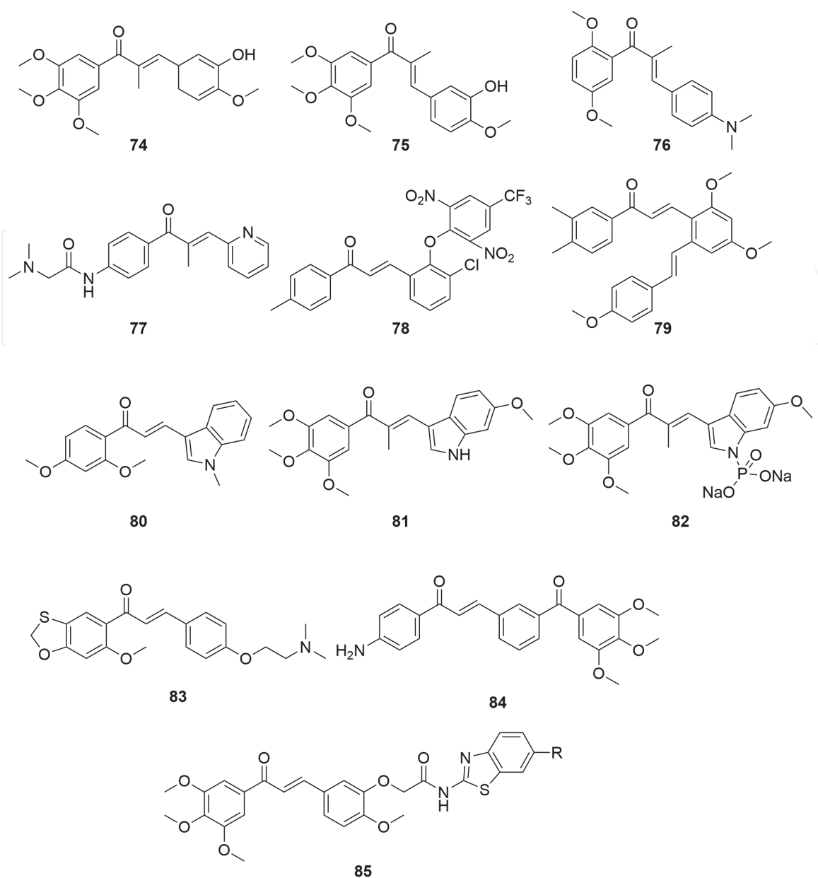
Figure 20. Chalcones computationally predicted to target tubulin [81, 82].
