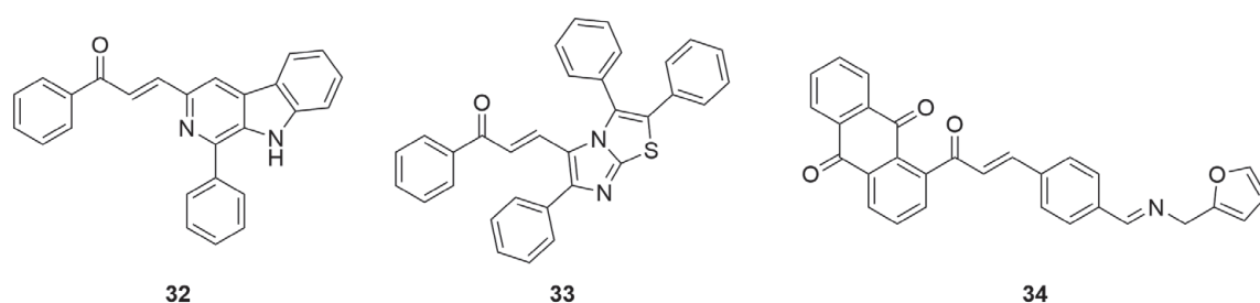
Figure 11. Representatives of fused chalcone analogues [54].
