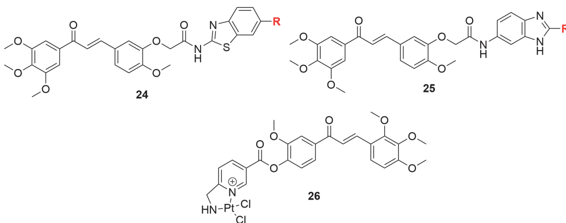
Figure 8. Selected ester and ether-linked chalcones [47, 48].
