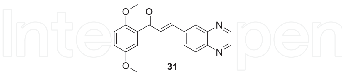
Figure 10. Chemical structure of chalcone 31 , ( E )-1-(2,5-dimethoxyphenyl)-3-(quinoxalin-6-yl)prop-2-en-1-one [53].
