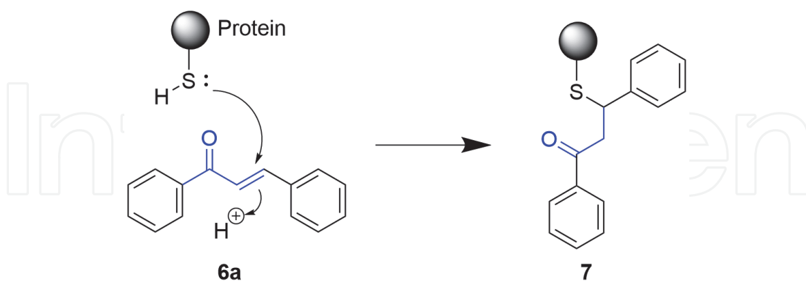
Figure 3. Michael addition of a chalcone ( 6a ) with cysteine to form the Michael adduct 7 .
