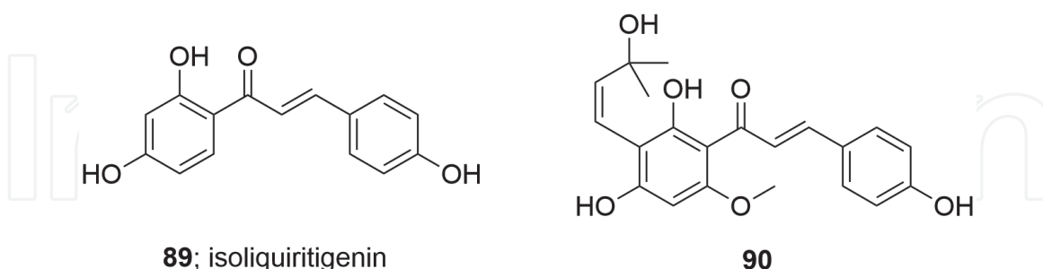
Figure 22. Chalcone isoliquiritigenin ( 89 ) and an analogue ( 90 ) with activity against the ER-positive breast cancer cell line (T-47D) [96, 97].
