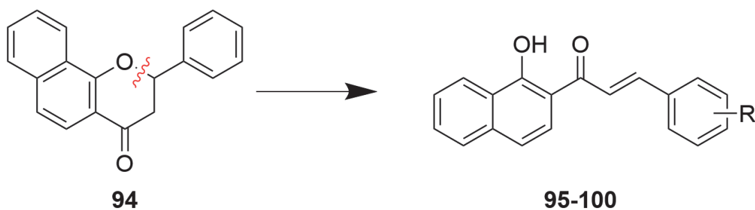
Figure 24. Structural modification of ANF leading to a family of CYP1B1 inhibitors displaying high levels of cytotoxicity, see Table 3 for details of “R” [99].
