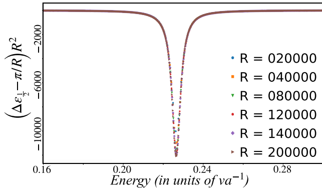
FIG. 4. Plot of \Delta\varepsilon_{1/2} = \varepsilon_{n+1}^{1/2} - \varepsilon_n^{1/2} , the nearest-level spacings for a spherical impurity with u = 3.1867 calculated from the numerically found solutions of the boundary condition [Eq. (B3)]. The data points are represented as R^2 \times (\Delta\varepsilon_{1/2} - \pi R^{-1}) , such that a collapse of different values of R is achieved. This collapse indicates that \Delta\varepsilon_{1/2}(R, \varepsilon, u) \approx \pi R^{-1} - f(\varepsilon, u)R^{-2} in the presence of an impurity. R is measured in units of b .
