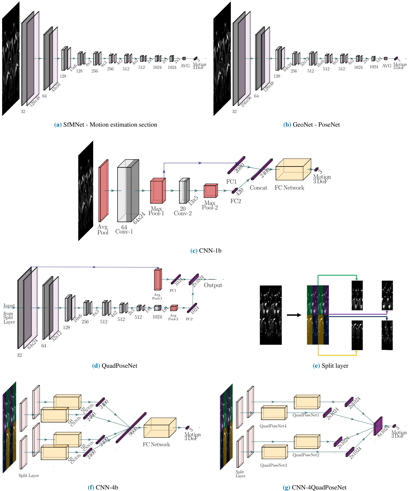
FIGURE 5: DL architectures for estimation of 3 DoF of position and orientation of an underwater platform using acoustic images.
