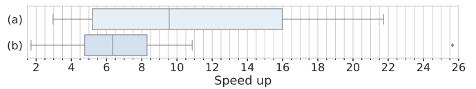
Fig. 11: (a) Speed-ups for PPP2 (aug) compared to TTK at 68 cores on KNL on 3D datasets. (b) Speed-ups for PPP2 (aug) on GPU compared to the best runtime for TTK on Haswell on 3D datasets. See also Supplements O and P for details.
