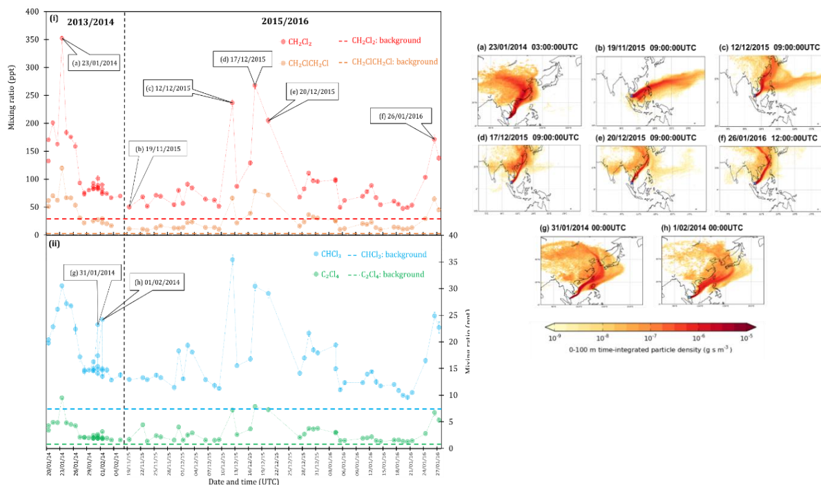
Figure 1. Left panel, Mixing ratios (ppt) of the four chlorinated VSLs in 68 air samples collected at Bachok during the Northern Hemisphere winters, 2013/2014 and 2015/2016. Right panel, (a) to (f): NAME footprint maps generated from a back-trajectory analysis indicating the likely origin of the air sampled at Bachok, with the darker colours indicating greater influence.
