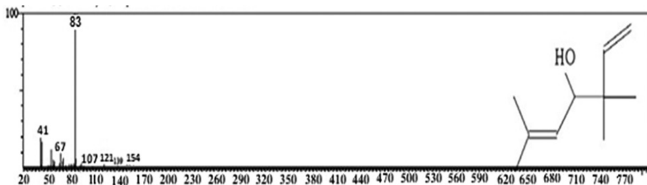
Fig. 5. A typical gas chromatogram of the artemisia alcohol.
