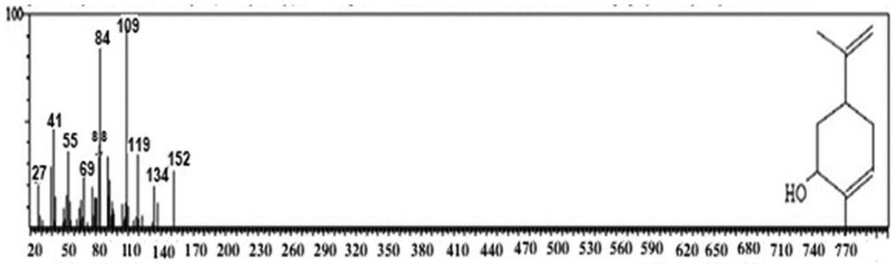
Fig. 6. A typical gas chromatogram of the trans-carveol.
