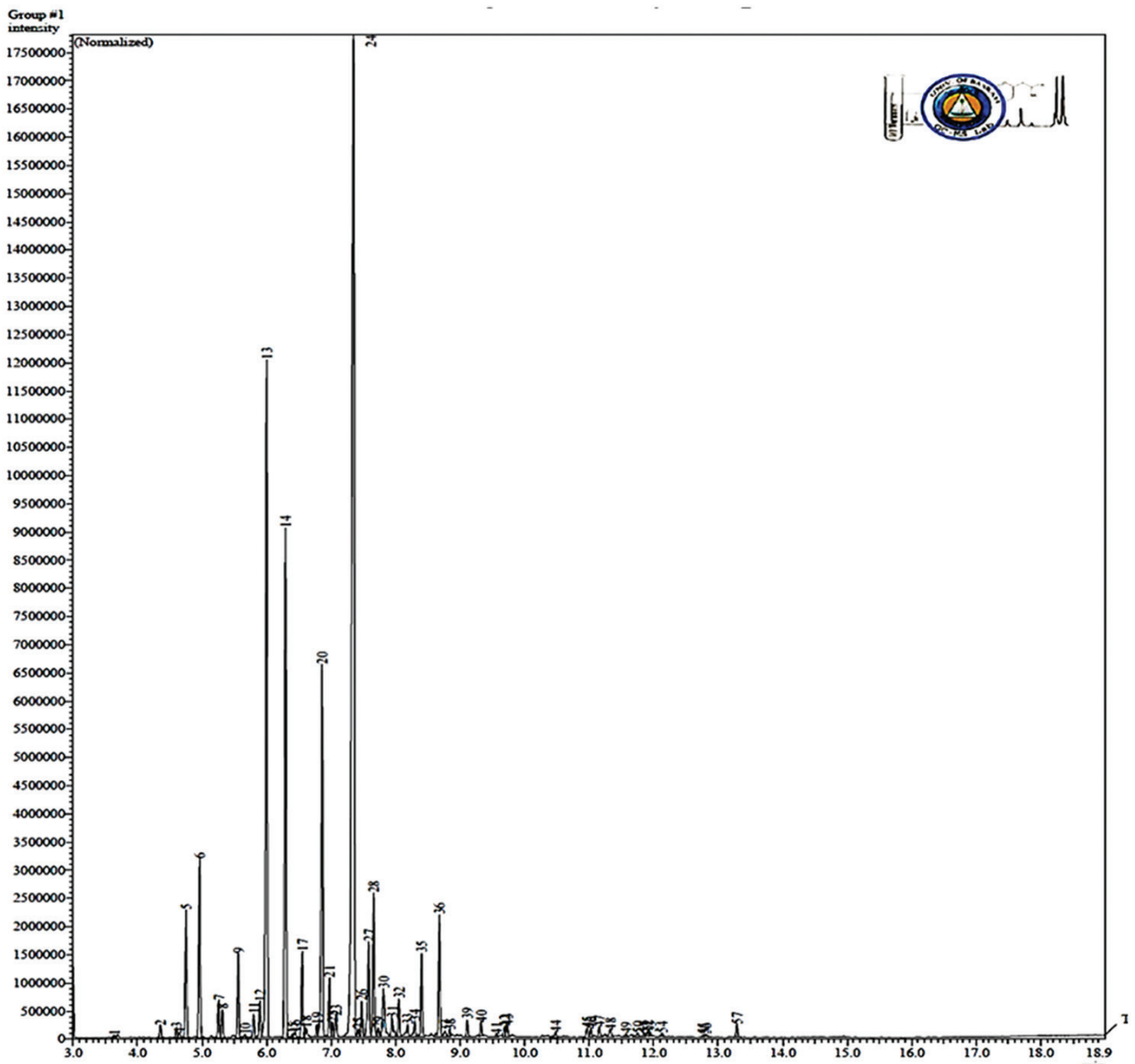
Fig. 7. Chromatogram of essential oil of Achillea fragrantissima leaves.
