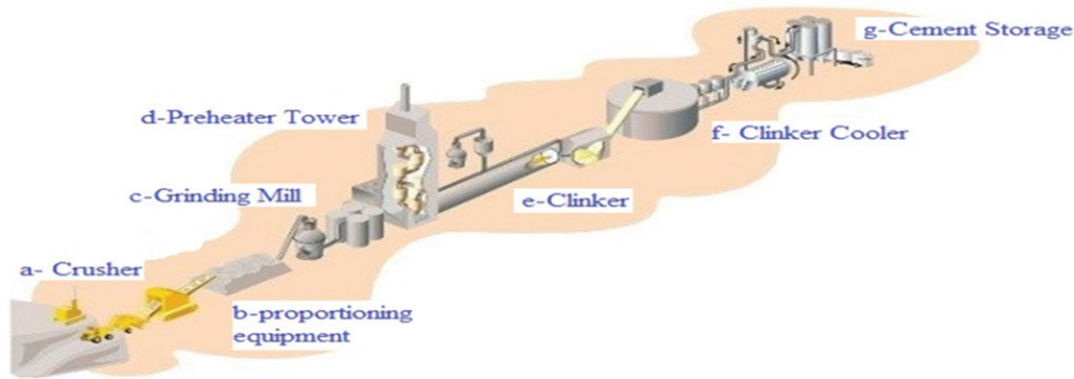
Fig. 1. Diagram of cement plant sectors of Lafarge association that established and reconstructed Bazian and Tasluja cement plants (CPs). The mass CP design is near to the other two plants (Holcim, 2016).
