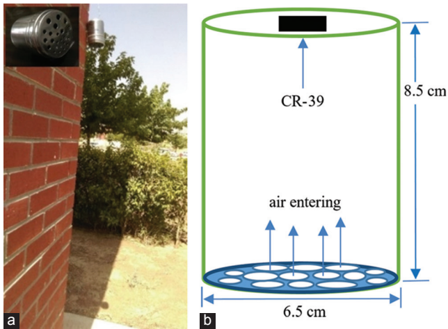
Fig. 2. Pinholes dosimeter containing CR-39 detector; (a) Dosimeter in situ (background) location and (b) diagram of the dosimeter.
