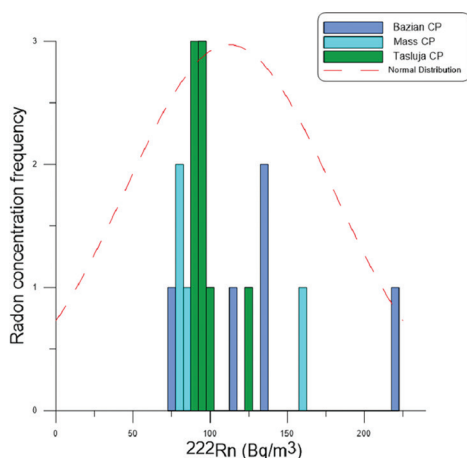
Fig. 3. Frequency distribution of the radon concentration in Bq m -3 for all sectors of the three cement plants
