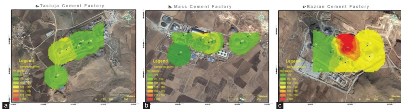
Fig. 4. (a-c) Landscape map of the investigated area to define radon concentration level of the sectors. (a) Tasluja cement plant (CP), (b) Mass CP, (c) Bazian CP.
