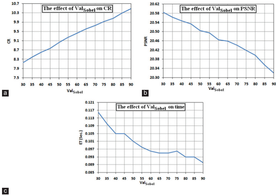
Fig. 5. (a-c) The effect Val Sobel .
