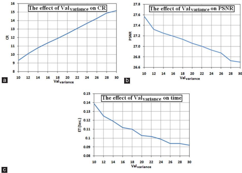
Fig. 7. (a-c) The effect Val_{variance} .
