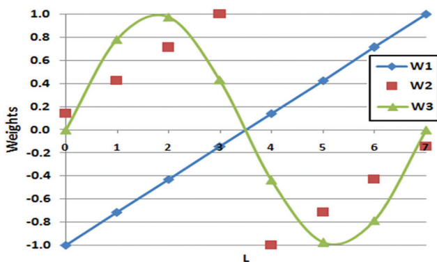
Fig. 1. The proposed weights.
