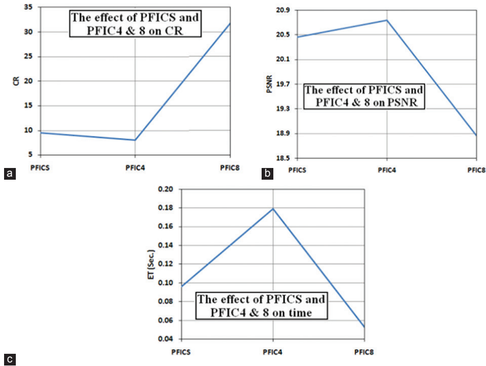
Fig. 6. (a-c) The effect of proposed variable partitioning scheme using Sobel with fixed one.
