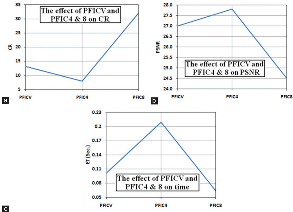
Fig. 8. (a-c) The effect of the proposed variable partitioning scheme using max variance with fixed one.
