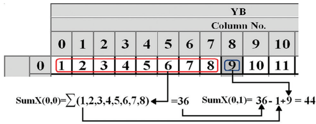
Fig. 2. Shows simple example of how the value of SumX(0,0) and SumX(0,1) had been computed for row sample when block length (L) equal to 8.
