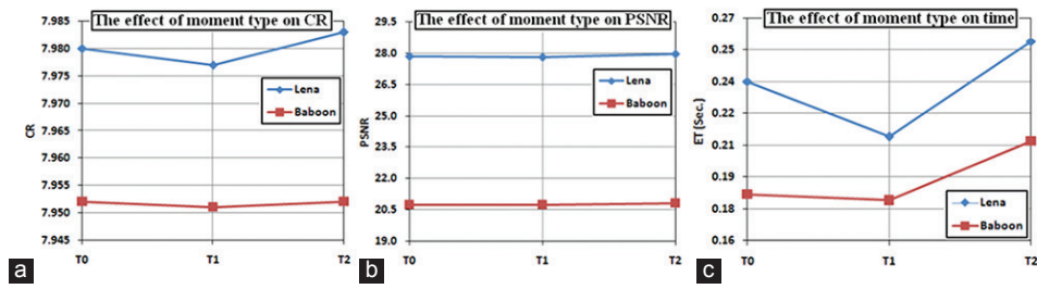
Fig. 4. (a-c) The effect of moment type with test images.
