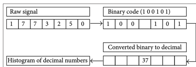
Fig. 1. One-dimensional local binary pattern, number of neighbors ( p=6 ).
