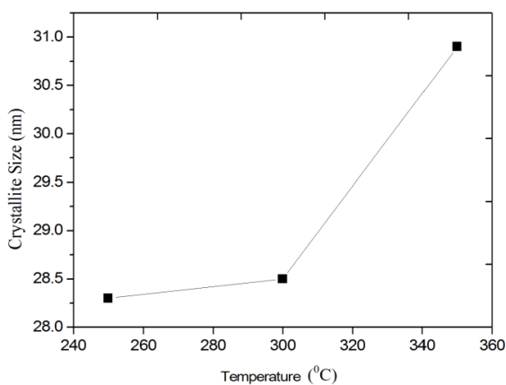
Fig. 4. Crystalline grain sizes as a function of substrate temperatures.
