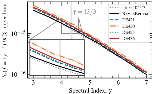
Figure 2. GWB amplitude 95% upper limit for an uncorrelated common process (model 2A) as a function of spectral index \gamma (see Equation (5)) for the JPL ephemerides and for BAYESEPHM. The dotted curve shows a power-law fit to the BAYESEPHM curve, which is consistent with a similar fit in NG9b.
