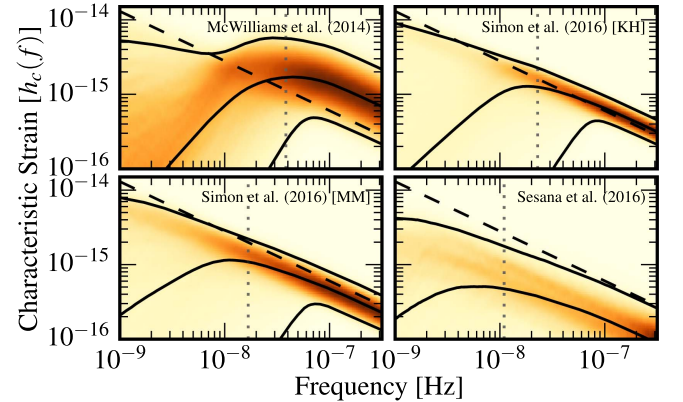
Figure 9. Posterior density plots of broken power-law GWB spectra, as constrained by the 11 year data set, adopting high-frequency A_{\text{GWB}} priors from MOP14, Simon & Burke-Spolaor (2016), and S16. At each frequency, a thin vertical segment of the plot should be understood as a density plot of the characteristic strain; the solid lines mark the 2.5%, 50%, and 97.5% quantiles, the dashed line shows the \gamma = 13/3 unbroken power-law upper limit, and the vertical dotted lines show the median f_{\text{bend}} values. All plots were produced for a spatially uncorrelated common GWB process. Larger values of A_{\text{GWB}} induce stronger turnovers at higher frequencies (e.g., MOP14 has a median value (50% quantile) of f_{\text{bend}} that is more than three times that of Sesana et al. 2016).
