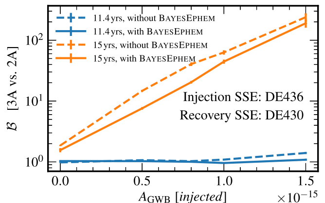
Figure 6. Model 3A-versus-2A (spatial correlation) Bayes factors for a set of simulated 15 year data sets with GWB injections at different levels. We analyze the full data sets (orange lines) as well as their 11.4 year “slices” (blue), both by adopting the “wrong” ephemeris (dashed) and by employing BAYESEPHM to marginalize over SSE errors (solid). We conclude that BAYESEPHM will not impede the ability of PTAs to make a definitive detection in the near future (see main text).
