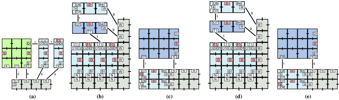
Figure 4: (a) The start gadget attaches. C1 + N = 2 + 9 \geq \tau = 10 . The first mold gadget attaches, cooperatively, to the start gadget and the input shape. O1 + N = 1 + 9 \geq \tau . The second mold gadget attaches, cooperatively, to the previous mold gadget and the input shape. O2 + N = 1 + 9 \geq \tau . (b) A concave corner of the assembly. The North→West corner gadget attaches. T1 + W = 1 + 9 \geq \tau . A mold gadget attaches. O7 + W = 1 + 9 \geq \tau . (c) A convex corner of the assembly. The West→North corner gadget attaches. O7 + N = 1 + 9 \geq \tau . (d) A type-2 concave corner of the assembly. The type-2 North→West corner gadget attaches. T1 + W = 1 + 9 \geq \tau . An mold gadget attaches. O7 + W = 1 + 9 \geq \tau . (e) An convex corner of the assembly. The West→North corner gadget attaches. O8 + N = 1 + 9 \geq \tau .
