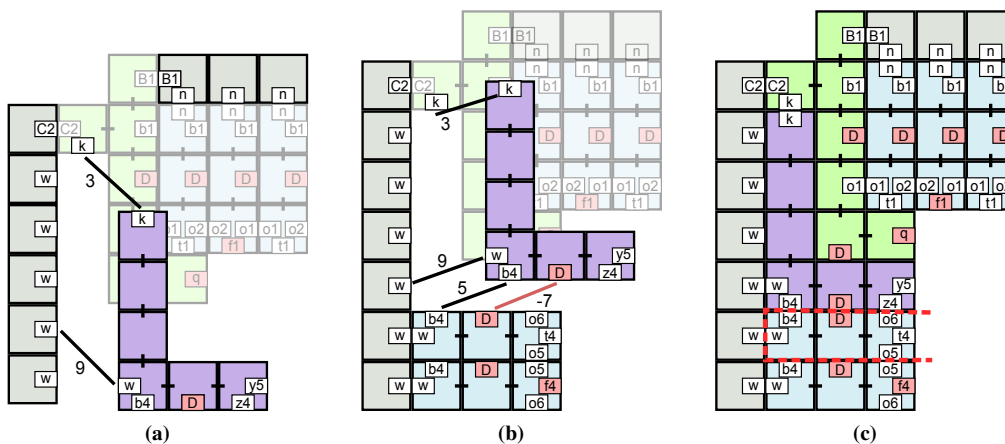
Figure 12: The inner pre-drilling process begins. (a) Case 1: The inner mold process has not completed and the inner pre-drill gadget binds cooperatively to the FRAME and the inner start gadget. w + k = 9 + 3 \geq \tau . (b) Case 2: The inner mold process has completed and the inner pre-drill gadget binds cooperatively to the FRAME, inner start gadget, and an inner mold gadget. w + k + b4 + D = 9 + 3 + 5 - 7 \geq \tau . (c) The inner pre-drill gadget prevents any inner mold gadget from attaching to its south and destabilizes any inner mold gadget that may have been in that space. b4 + o5 + w + D = 5 + 1 + 9 - 7 < \tau .
