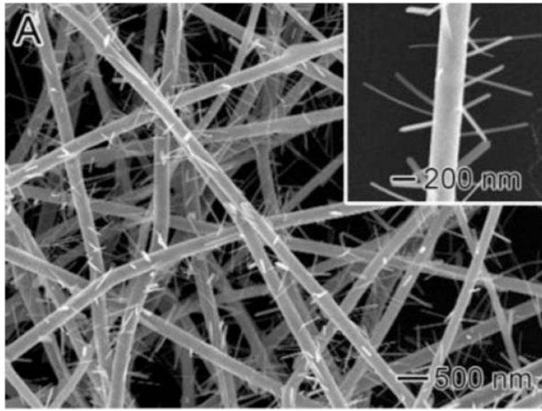
Figure 17. SEM images of (A) V_2O_5 - TiO_2 - Ta_2O_5 nanofibers. Reproduced with permission. [192] Copyright 2006, American Chemical Society.
