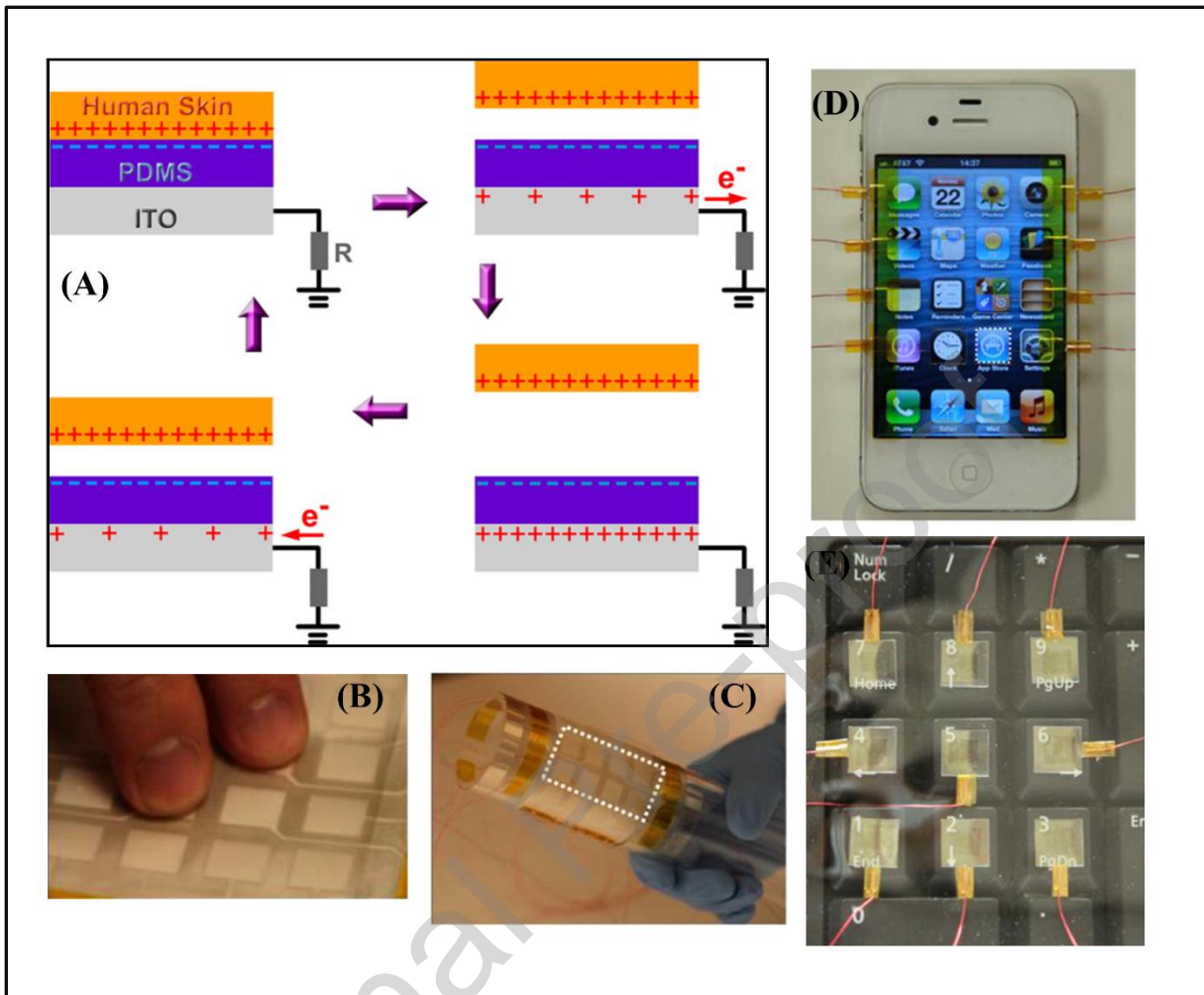
Figure 2.1: (A) The electricity generating cycle for TENG through contact electrification between PDMS and human skin, (B) small squares of this TENG has been organized into a grid to map out the exact location of pressure by finger pressing, (C) this flexible grid is attached to an acrylic tube to measure grip strength, (D) 1 cm x 1 cm TENG cubes attached to the screen of a cellphone, also (E) attached to the number pad, in order to harvest energy from daily cellphone activities.
