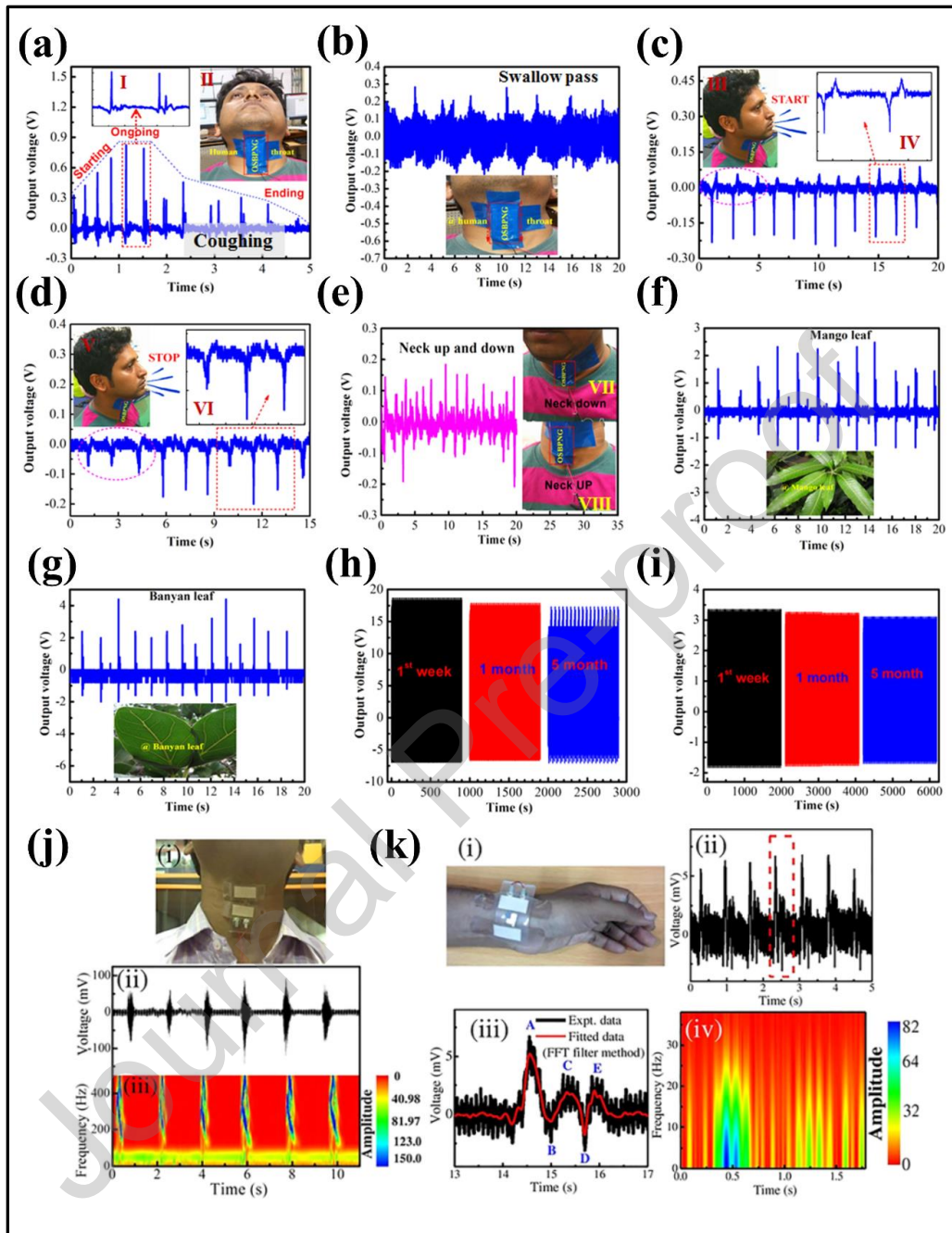
Figure 3.3: Output voltage of onion skin based nanogenerator attached to the throat when (a) coughing, (b) swallowing, (c) saying “start”, (d) saying “stop”, (e) nodding up and down. The voltage output when a (f) mango leaf and (g) banyan leaf was dropped, showing the sensitivity of the generator. The stability of the nanogenerator when (h) hand punching and (i) sewing machine vibration. A prawn shell based nanogenerator attached to the throat (j-i) with its corresponding output values (j-ii). A prawn shell based nanogenerator attached to the wrist (k-i), with its corresponding voltage outputs of (j-ii) wrist pulse vibration. The data was enlarged, and noise was removed (k-iii) and an STFT spectrogram was selected for a single pulse wave (k-iv).
