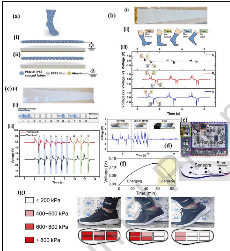
Figure 4.4: (a) A schematic diagram of the modified sock and the PTFE film with aluminum electrodes (i, ii). The device has two modes of electrical connections, the (i) sock connection and the (ii) Al/PTFE connection. (b) The device can help analyze footsteps. (i) A photograph of the PTFE laid on the floor like a carpet. The phases of a footstep (ii) can be reflected by the (iii) sock and PTFE's output. Three participants, a (A) 90 kg male, (B) 70 kg male, and (c) 60 kg male, tested the output. (c) The sock can also determine the direction and speed of walking. (i) A photograph of a PTFE modified with six pairs of designed aluminum electrodes with two electrodes. This design could determine the (ii) walking direction and the (iii) speed and distance walked. (d) The output for normal walking, loss of stride length walking (more peaks for more frequent steps), and freezing of gait, which can be used to help diagnose a Parkinson's disease patient. PVDF-based HBNG used to harvest energy from footsteps. (e) A circuit diagram of the wireless sensors system with the outputs of three rectified tribo-piezo hybrid nanogenerators (TPHG) being used to charge a Li-battery powering a wireless pressure sensor. (f) The charging and discharging process for the Li-battery is shown. (g) Through the wireless pressure sensor, the pressure on the bottom of the feet can be mapped [62, 63].
