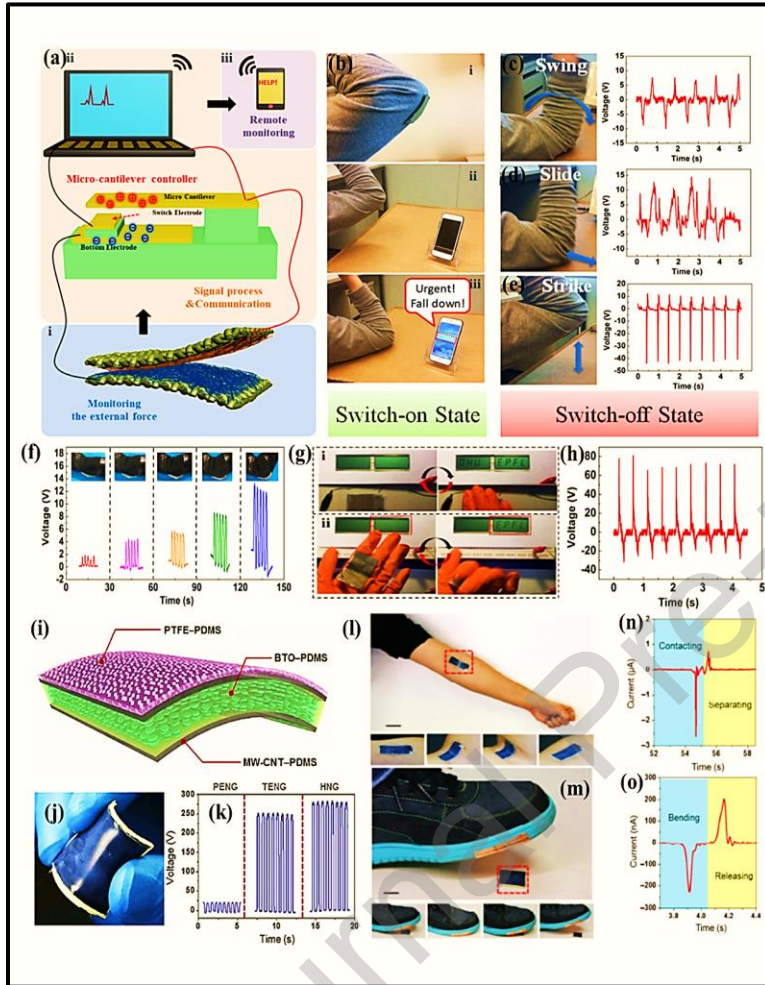
Figure 5.1: (a) An illustration of a fall alert system by fiber based HBNG. The device was tested attached to the elbow (b), and a simulated fall by dropping the elbow against the table (b ii) resulted in an emergency message (iii). Additionally, the device can also be used in energy harvesting while the electrical output does not reach the threshold, and the outputs of common motions like a swing (c), slide (d), and strike (e) are shown. (f) Different voltage outputs for different bending angles from 101^\circ to 146^\circ for the HBNG when attached to the elbow. The device was used to power LCDs with tapping (g i) and with folding (g ii). The voltage output with \sim 2 Hz frequency hand tapping reached 78 V (h). (i) A schematic diagram of a HBNG fabricated using multilayered nanocomposite materials with a PTFE nanoparticle and PDMS matrix top layer. The device is flexible and can be bent (j). The output was recorded (k), and the hybrid nanogenerator output (HNG) exceeded both the TENG and PENG outputs. (l) The hybrid nanogenerator used to harvest energy from the flexion and extension of the elbow joint and the output was recorded (o). The HBNG could also harvest energy from footsteps as shown in (m), and (n) shows the output. [27, 67]
