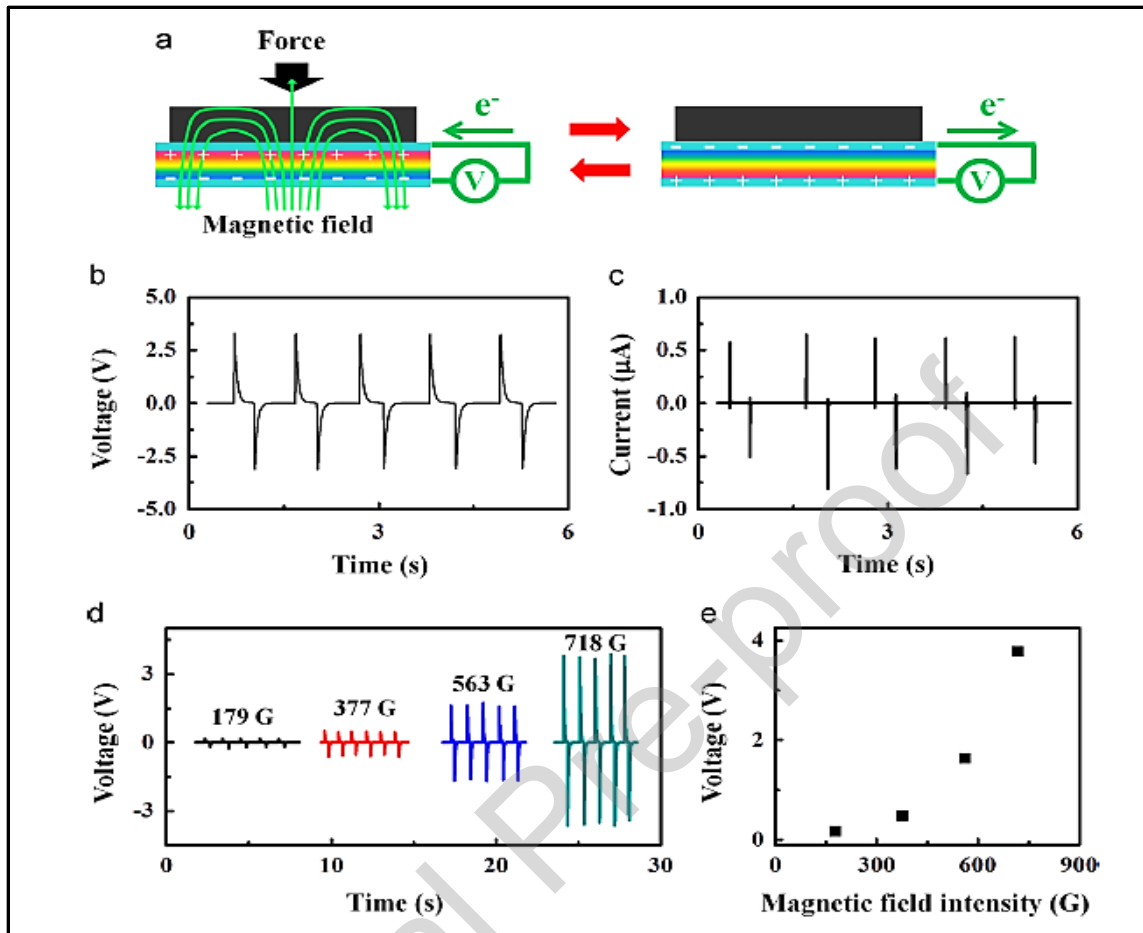
Figure 3.4: (a) Schematic diagram of WLNG and its working mechanism, (b) Output voltage of the WLNG, (c) Output current of the WLNG, (d) Voltage vs time plotted for different magnetic field intensities, and (e) peak output voltage plotted vs magnetic field intensity.
