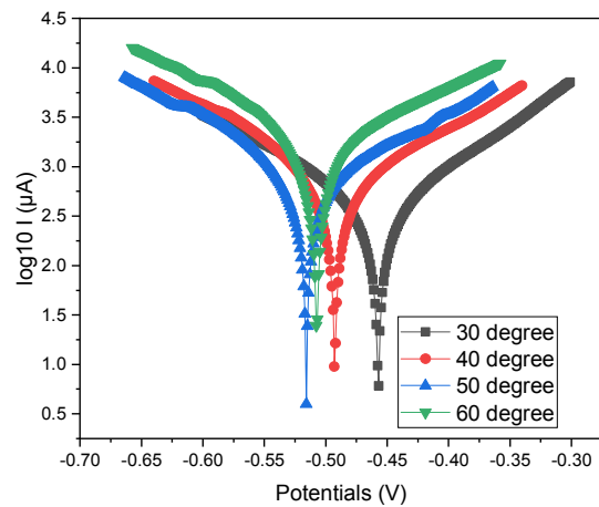
Figure 6. Tafel plots of mild steel specimen in 1.0M HCl at different temperature and fixed concentration of methanol extract of Alchornea laxiflora leaves.
