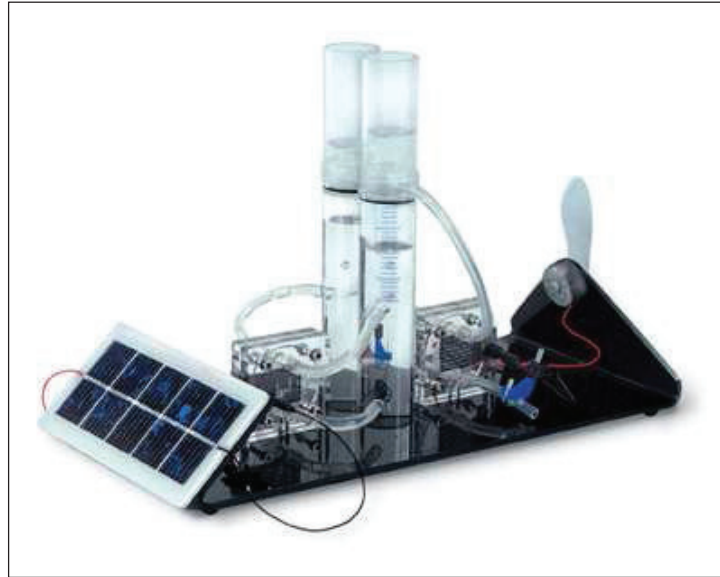
Figure 1. Testing Apparatus
