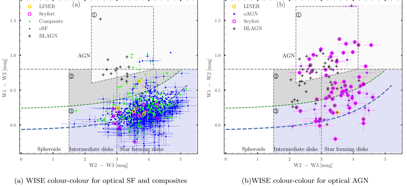
Figure 9. The BPT [O\text{III}]\lambda 5007/H\beta vs. [N\text{II}]\lambda 6583/H\alpha classified galaxies from Figure 7 plotted in the WISE colour-colour diagram. Those also classified as Seyferts and LINERs from Figure 6 are over-plotted in magenta and gold circles, respectively. The dashed blue and green lines are the fit to the sequence of galaxies (equation 1) seen at low W1 - W2 colour and the 2\sigma RMS curve of the fit. The AGN box is from Jarrett et al. 2011). The diagram is separated into 3 zones: The Zone 1, 2 and 3 are the respective locations of the WISE powerful AGN, the low power AGN and finally the non-AGN zone mostly populated by star-forming galaxies. The majority of the galaxies classified as LINERs using [S\text{II}] are classified as composites or SF based on the [N\text{II}] line while the Seyferts are generally classified as AGN using [N\text{II}] . The composites (green) occupy the star-forming zone. The majority of the optical non-AGNs in the WISE AGN zone are broad-lines for which using the line ratio is problematic. The optical star-forming and composites are presented in (a) and optical AGN in (b); they are separated for clarity.
