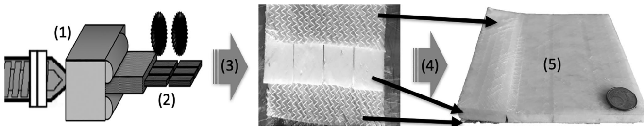
FIGURE 3 Scheme of sample preparation procedure with (1) foam extrusion and calibration, (2) removal of skin and preparation of 100 mm × 25 mm × 10 mm samples from the core region, (3) packing of sandwiches laminates, (4) VARI proceeding, and (5) final 100 mm × 100 mm × 13 mm cone calorimetry sample (the sample presented was prepared with one open side for proper illustration of final layup GF-core-GF)
