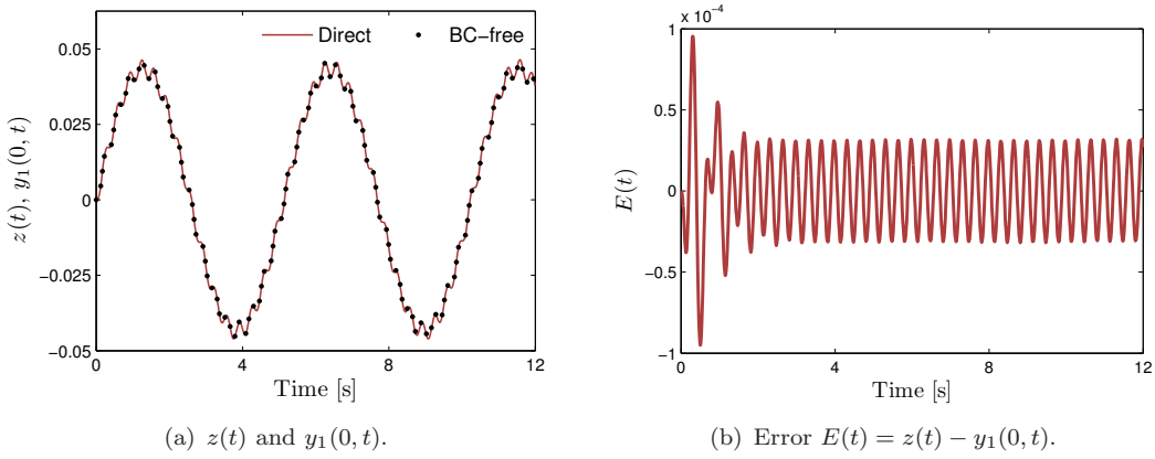
Figure 4. Comparison of direct numerical solution z(t) and solution obtained using the Galerkin method y_1(0, t) for (34). The parameters are b_1 = b_4 = 0 , b_2 = 1.5 , b_3 = 0.1 , \alpha = F = 1 , \beta = 0.5 , \omega = 6\pi , and N = 7 .
