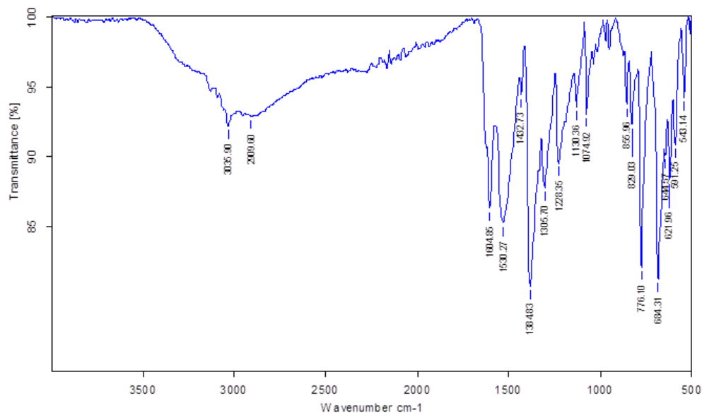
Figure S3. FT-IR (neat) spectrum of compound 3 .
