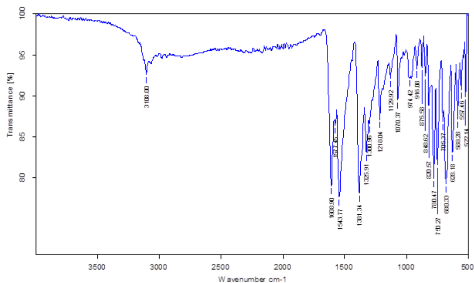
Figure S6. FT-IR (neat) spectrum of compound 6 .
