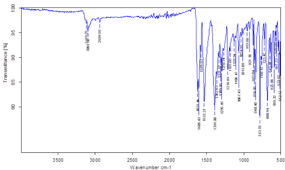
Figure S6. FT-IR (neat) spectrum of compound 6 .
