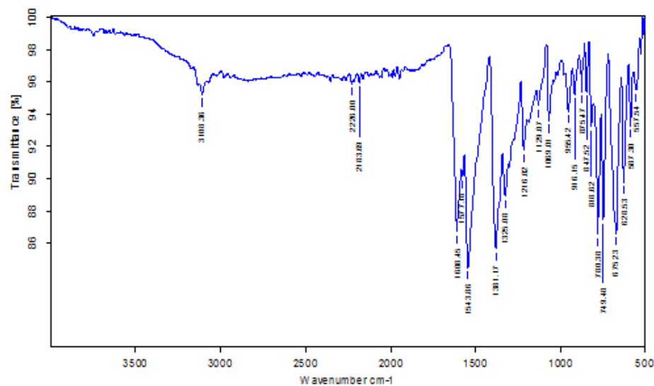
Figure S2. FT-IR (neat) spectrum of compound 2 .
