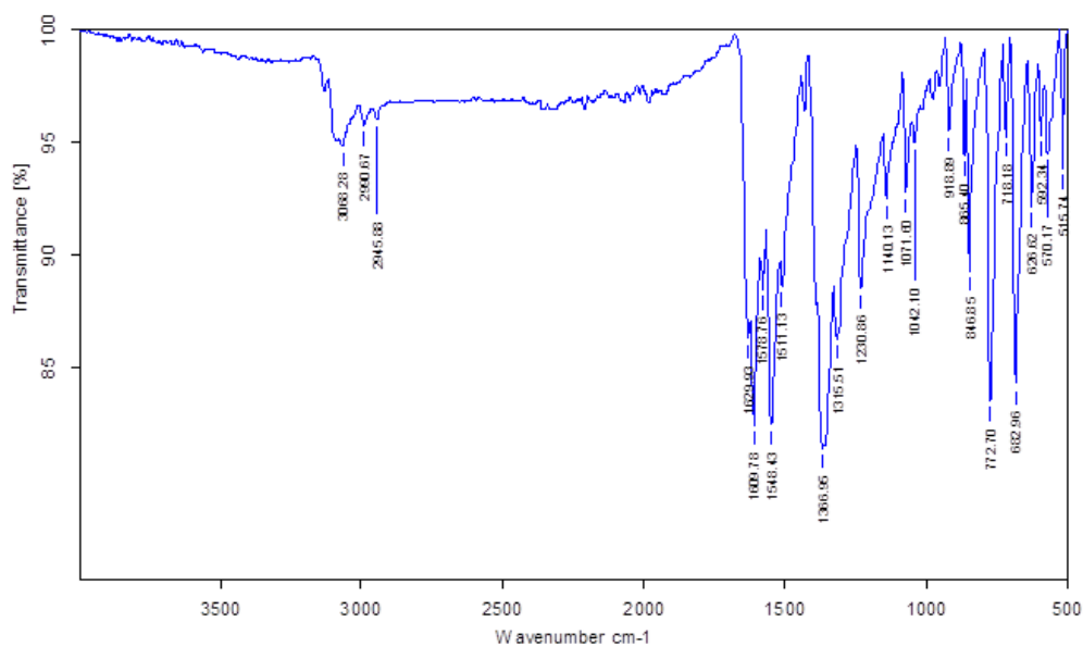
Figure S4. FT-IR (neat) spectrum of compound 4 .
