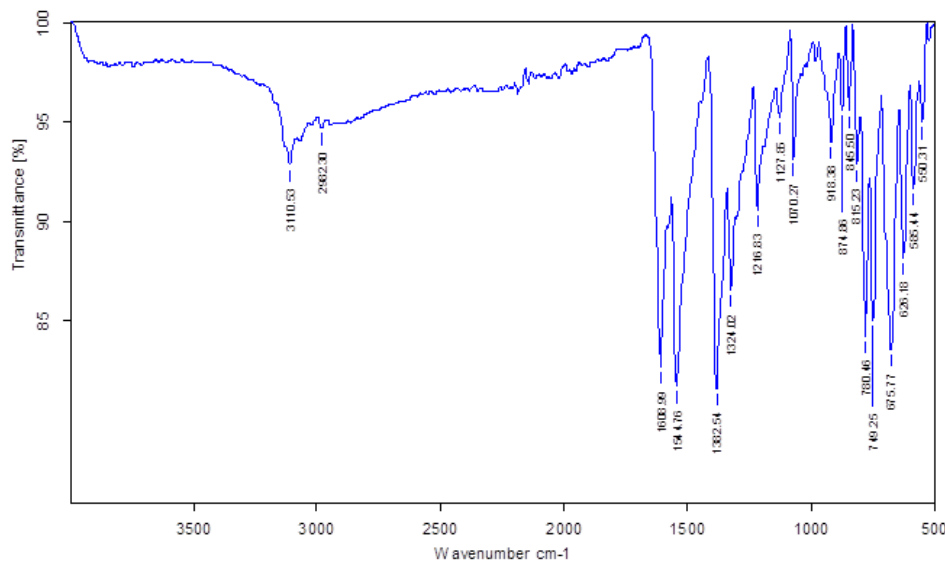
Figure S1. FT-IR (neat) spectrum of compound 1 .
