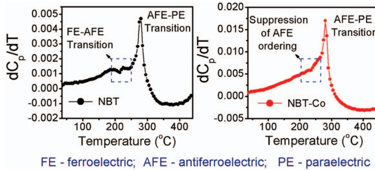
FIG. 6. The variation in dC_p/dT as a function of T(^{\circ}\text{C}) plot for (a) NBT and (b) NBT-Co sample indicating the suppression of AFE ordering due to Co-substitution (100kHz data was depicted for both the samples).
