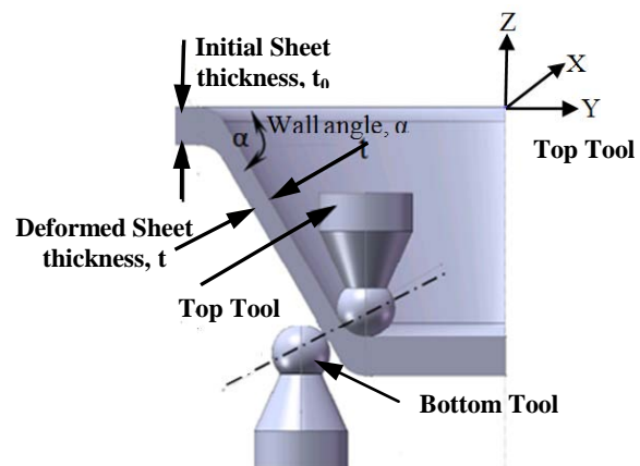
Fig 4: Normal tool configuration
