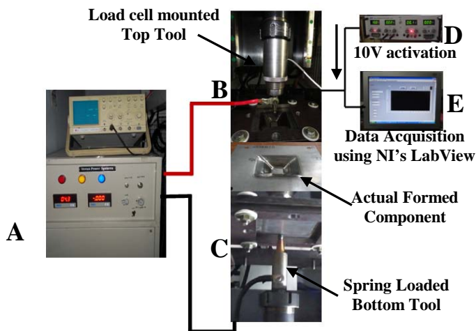
Fig 2: Actual experimental set-up used in the present study
