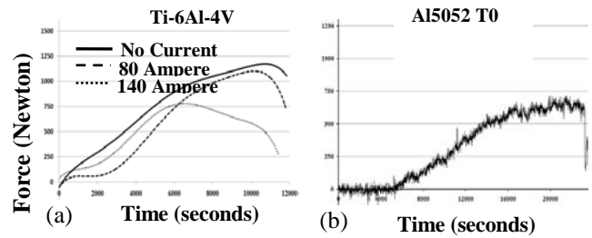
Fig 8: (a) Load measurement for 30 degree truncated pyramid of Titanium alloy (frequency: 55 Hz, On-time: 3ms, Max. temp: around 47° C with 140amps current) (b) Load curve for 30 degree truncated pyramid of Al5052T0 without electro-pulsing
