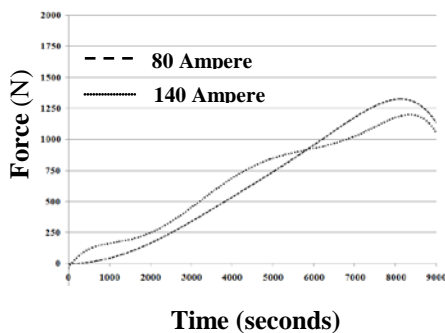
Fig 11: Force data plot for 45° pyramidal component failed after approx. 12 mm depth
