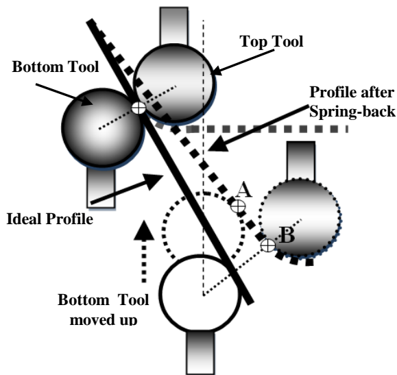
Fig 10: Effect of spring back on normal tool configuration
