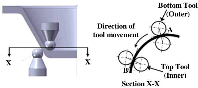
Fig 6: Schematic depiction of synchronization of top and bottom tool during forming
