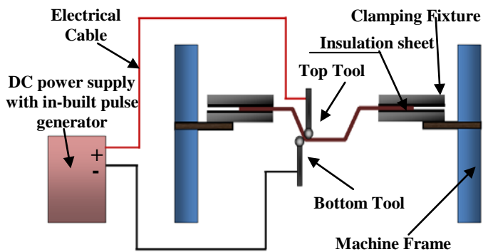
Fig 1: Schematic of experimental set-up used for Incremental Electro-plastic deformation
