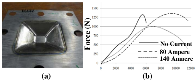
Fig 14: (a) Actual picture of 45° pyramidal component formed at 140 ampere current (b) Force data for 45° pyramidal component at 0, 80 and 140 ampere current
