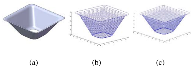
Fig 5: (a) CAD Model (b) Contour Tool path (c) Helical Tool path
