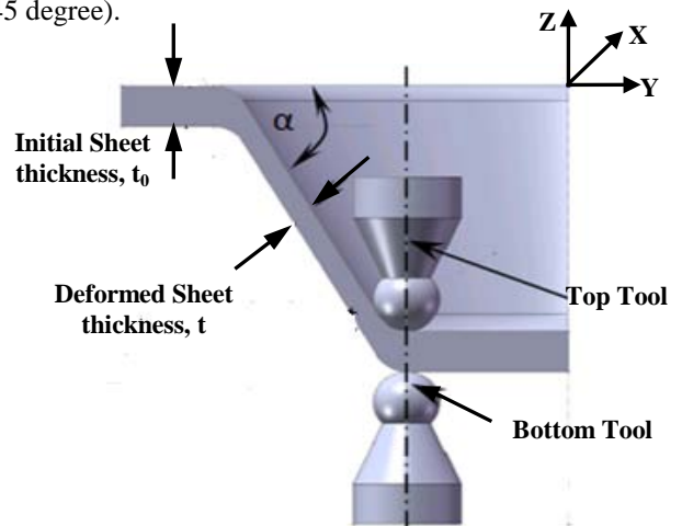
Fig 12: Align Tool Configuration
