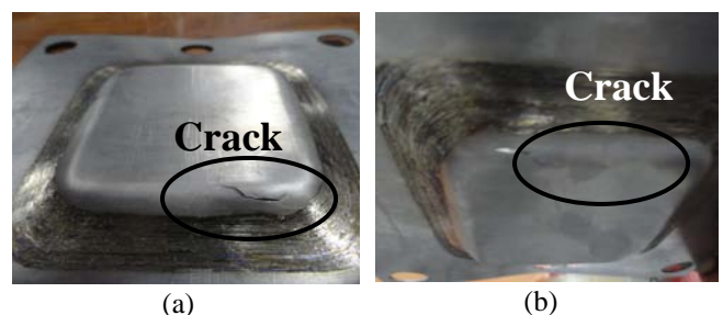
Fig 9: Picture of failed 45° pyramidal component and resulted crack
