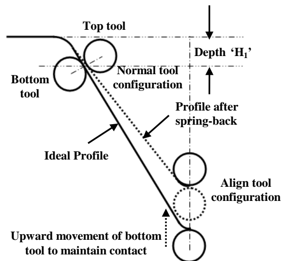
Fig 13: Mixed tool configuration
