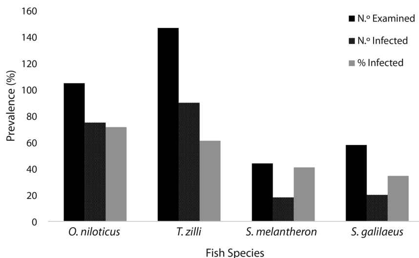
Fig. 1. Infection Rate of Fish Hosts.
