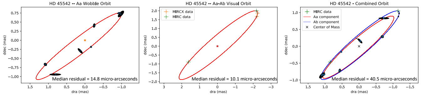
Figure 14. (Left) Subtracting out the binary motion of \nu Gem, we show the fit results of the inner wobble of the primary star induced by the \sim 54 day companion. Here we are fitting only to the outer binary motion + wobble. (Center) We also detect flux from the Ab component in four MIRC-X epochs, and in two epochs of MIRC data. We plot the best fit orbit when fitting only to this Aa-Ab pair. Visually, one can see that the best-fit orbit does not agree well with the orbit fit of the wobble motion alone. The wobble motion prefers a higher eccentricity orbit than that derived from the visual data alone, with a significantly larger period. (Right) We show the combined fit, when coupling the wobble motion to the visual orbit. The median residual of the orbit increases, due to the residuals from the wobble motion. This extra residual is potentially due to time-varying resolved structure from the Be star disk, or additional companions in the system.
