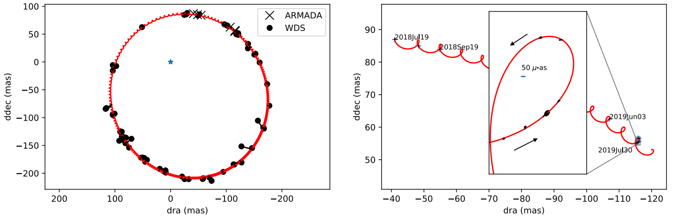
Figure 10. (Left) We show the outer binary orbit of \alpha Del as the Ba component moves relative to the A component fixed at the origin. Though the WDS data do not have enough precision to help constrain the inner orbit, we include these data in order to constrain the outer binary orbit. (Right) Showing only the new ARMADA data, clearly we detect an added astrometric wobble due to the presence of the Bb component.
