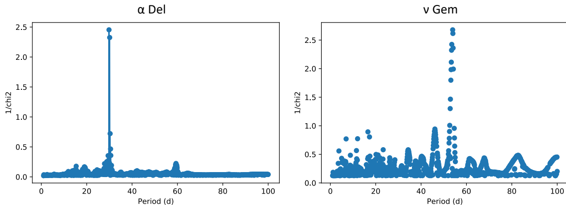
Figure 5. We show our period search results for the new detections of inner tertiary companions to binaries \alpha Del and \nu Gem. Since the period and eccentricity are nonlinear parameters in our orbit fits, we search for extra components by varying the period on a grid and searching for circular tertiary orbits. For \alpha Del we see a clear signal at a period of about 30 days, while \nu Gem shows a strong detection at a period of about 54 days. The reduced \chi^2 values are < 1 in these cases, as this search occurs before scaling the final ARMADA error bars.
