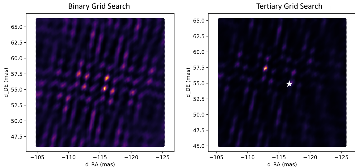
Figure 2. We show example chi-square maps for the 2019Jul30 epoch of \alpha Del. To search for flux from triple companions, we first perform a grid search for the brighter binary (left). Due to the signal from a tertiary companion, this initial \chi^2 map is quite messy. We then do a grid search for a third component, with a fit for the binary companion performed at each iteration (right). The location of the binary component is denoted by the star in the plot. Including this third component vastly improves the chi-square maps. Once we narrow in on the best solutions for each component on the grid, we perform a joint least-squares fit to refine the solutions.
