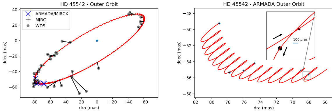
Figure 13. We detected the inner tertiary component to the system of B-type binary \nu Gem. We show the best fit to the ARMADA+WDS data for the outer binary pair - we zoom in to the ARMADA portion of the orbit to show that there is clearly an additional “wobble” to this binary motion.
