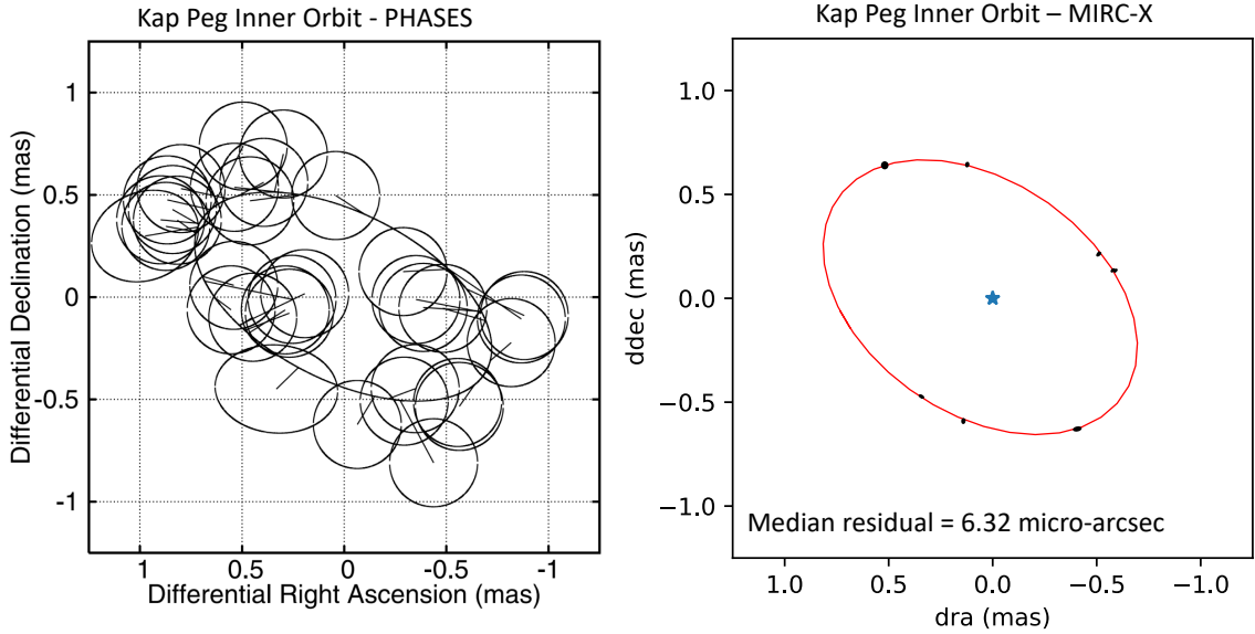
Figure 7. We show our best-fit orbit to the inner "wobble" of \kappa Peg due to the tertiary companion, after subtracting out the outer binary motion. We compare the results of the PHASES best-fit orbit from Muterspaugh et al. (2006) (left) to our MIRC-X+WDS fit (right). Over the \sim year time baseline of following this object with MIRC-X we are achieving a median residual level of 6.32 micro-arcseconds, which is very promising for our ultimate goal of detecting giant planets in binary systems with the ARMADA survey.
