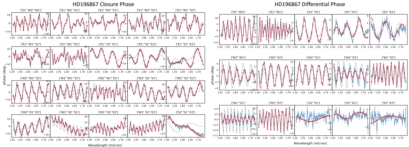
Figure 1. We show an example fit of our triple model to our observables closure and differential phase of \alpha Del from 2019Jul30. The two panels show our best fit (dashed red line with crosses) to closure phase (left) and differential phase (right). The dashed grey line shows the best-fit binary model, which is a significantly worse fit to our data than the triple model. Each square in the plots represents one of MIRC-X's 20 closing triangles or 15 baselines (the 6 telescopes are designated as E1-E2-W1-W2-S1-S2). This is a single 60-second measurement, of which we typically have \sim 10 per observation of a target.
