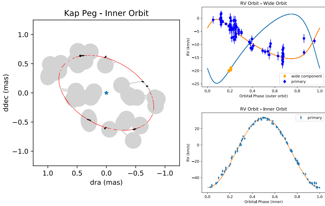
Figure 8. For a final orbital fit, we combine our new MIRC-X data with the historical data and PHASES/RV data presented in Muterspaugh et al. (2006). (Left) We plot the bright component going around the center-of-mass of the inner pair, once the outer binary motion is subtracted out. The light grey ellipses are data from PHASES, while the smaller black ellipses are the new data from MIRC-X. We show RV data of the primary and secondary phased to the outer orbital period of 11.6 years (upper right). Here the RV motion of the bright primary due to the inner companion is subtracted out. We also show data of the brighter component phased to the 5.9 day inner period (lower right).
