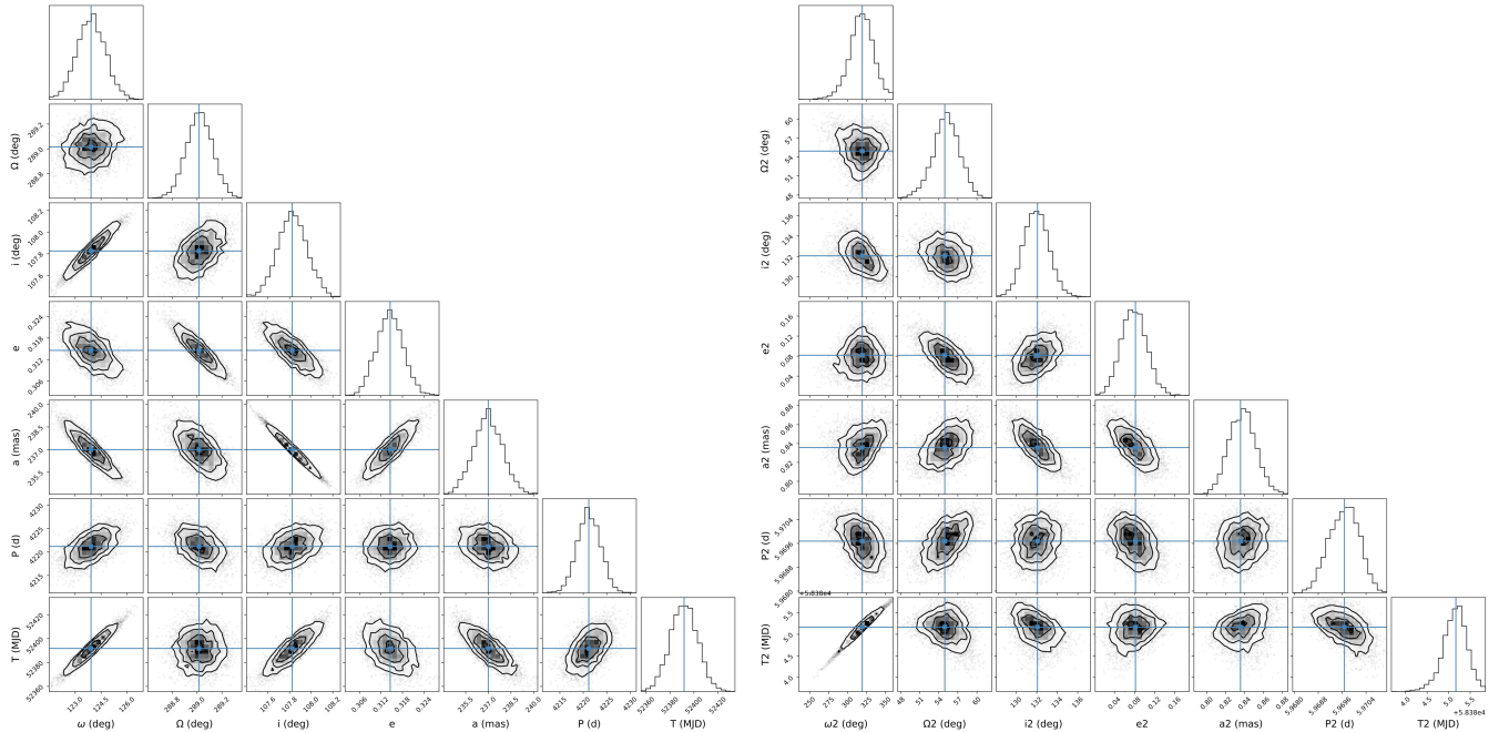
Figure 9. We show corner plots of the MCMC posterior distributions produced from emcee for the outer (left) and inner (right) orbital elements for \kappa Peg. Since the outer long-period orbit is less well-constrained than the short-period inner orbit, there are more obvious correlations between the parameters. Since the inner orbit is near circular, there is a strong correlation between \omega_2 and T_2 .
