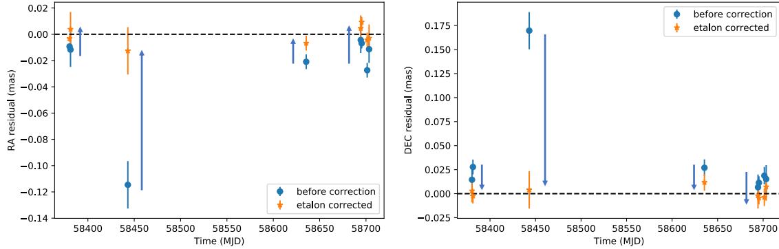
Figure 4. We show the R.A. and DEC residuals of \kappa Peg both before and after applying our etalon correction factor. The mean and median residual values both decrease, bringing us to our desired \sim 10 micro-arcsecond precision which is needed to eventually detect substellar companions. The most significant correction in this case is a single outlier point which was >100 micro-arcseconds off from the expected orbit before the etalon factor is applied.
