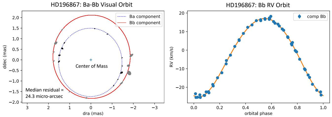
Figure 11. We subtract the outer orbit of \alpha Del to reveal the photocenter motion of the Ba component around the center-of-mass of the newly detected Ba-Bb system. Since we detect flux from the new Bb component, we can also show the Bb position. The motion of Ba+Bb about their center-of-mass allows us to work out the mass ratio of this inner pair, which in turn leads to measurements of all three masses in the system.
