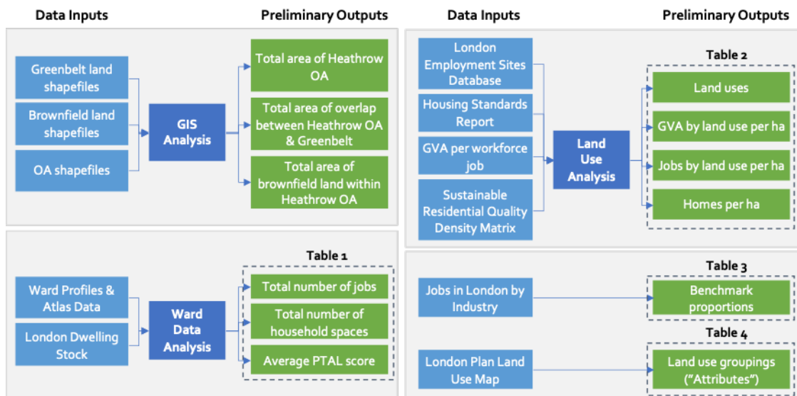
Figure 2: Data preparation analytical flowchart
