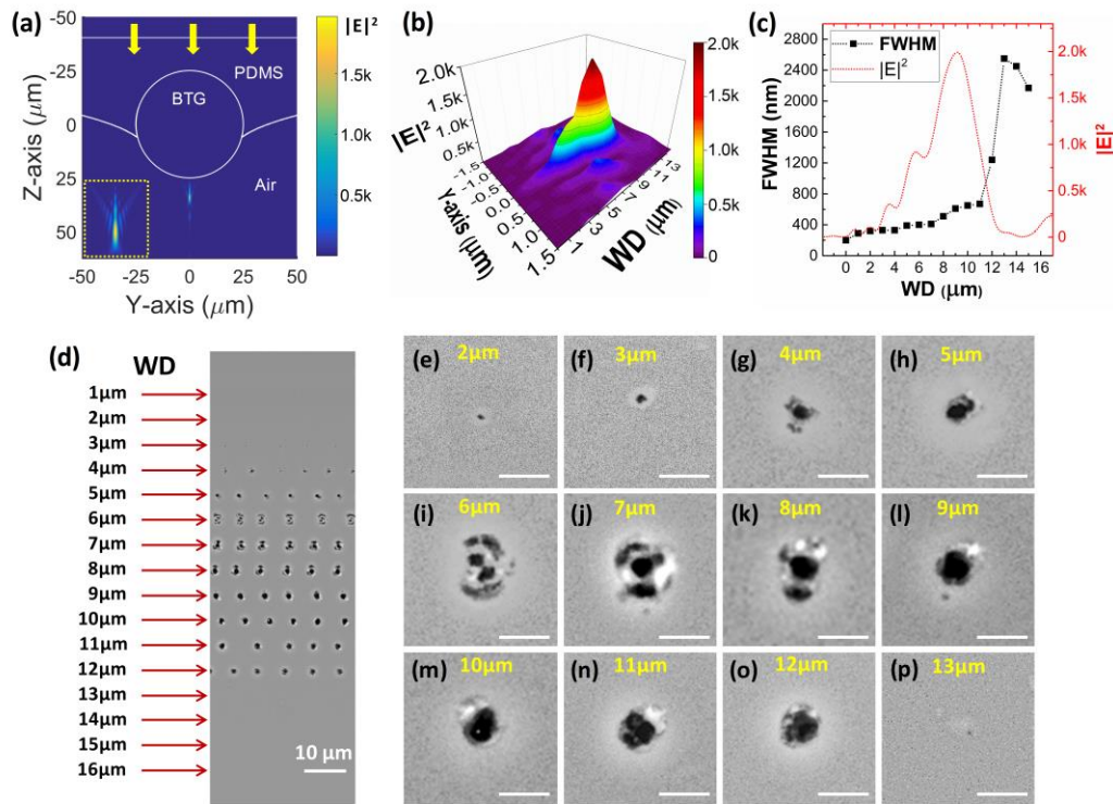
Fig. 2. Modelling of PCM lens focusing properties and experimental results of femtosecond laser machined feature size against WD. (a) Electric field intensity |E|^2 distribution of PCM lens across the YZ incident plane, the inset shows the enlarged view of focusing area. (b) Field distribution along y-axis and (c) FWHM and |E|^2 enhancement at different WD. (d) Femtosecond laser patterned feature at WD from 1 to 16 \mu\text{m} , and enlarged SEM images (e)-(p) at 2-13 \mu\text{m} distances, scale bar in (e)-(p) are 2 \mu\text{m} .
