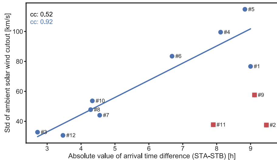
Figure 6. Standard deviation of the ambient solar wind versus the arrival time difference between STA and STB predictions. The Pearson correlation coefficient for all events under study (black) is calculated. In blue, we present the Pearson correlation coefficient and a linear fit when excluding the outliers (indicated by the red boxes), that is, flank hits (events #2 and #9) and the CME-CME interaction event (event #11). STA, STEREO Ahead; STB, STEREO Behind; CME, coronal mass ejection.
