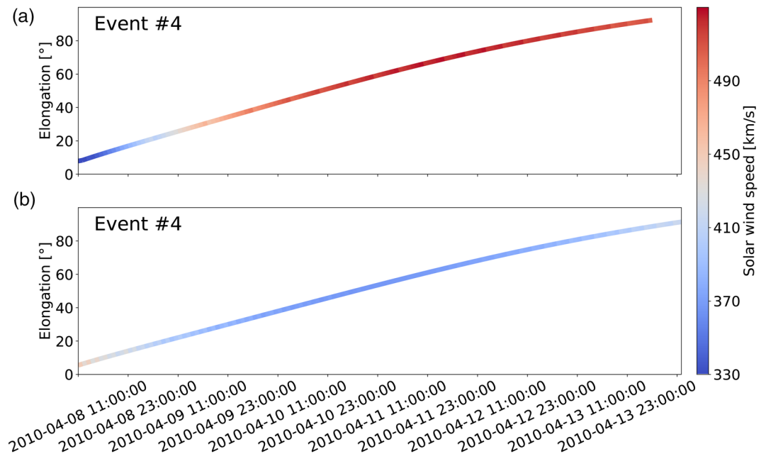
Figure 4. Ambient solar wind speed at the tangent points for event #4. Plotted are time series of the elongation angles of the tangent points as seen from STA (top panel) and STB (bottom panel) color-coded according to the speed of the ambient solar wind at that tangent point. STA, STEREO Ahead; STB, STEREO Behind.
