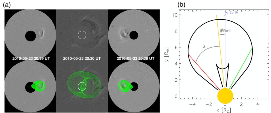
Figure 1. GCS reconstruction (left) and ecliptic cut of the wire frame (right) for event #5. (a) Top row from left to right: STB/COR2, LASCO/C2, STA/COR2. Bottom row: same as top row but with the GCS wire frame overlaid. (b) Ecliptic cut (black) of the GCS wire frame. Red and green lines show the boundaries selected by either EAGEL or the user. The yellow line defines the ecliptic propagation direction with respect to Earth, \phi_{\text{Earth}} , of the CME. The half width, \lambda , is the angle between one boundary and \phi_{\text{Earth}} . The blue arrow indicates the direction to Earth.
