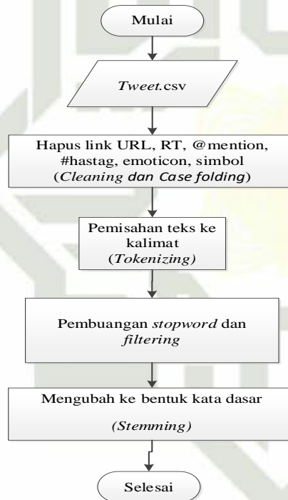
Gambar 3.2 Alur Preprocessing Text
