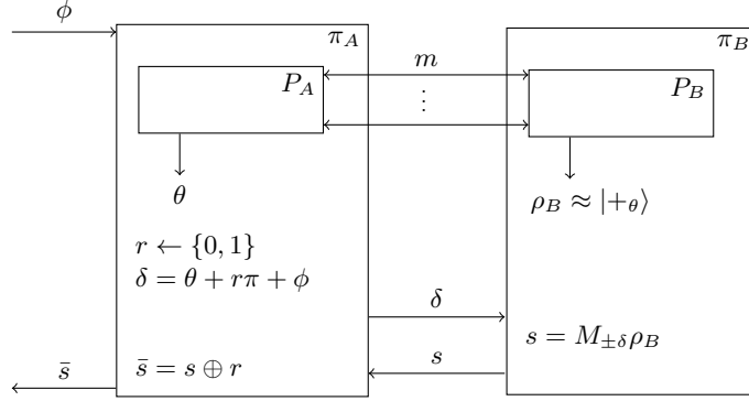
Fig. 5: UBQC with one qubit when both Alice and Bob follows the protocol honestly (see Protocol 1)
