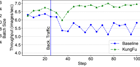
Fig. 5: Adaptive communication strategy (ResNet-50)
