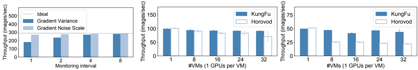
Fig. 8: Monitoring overhead
