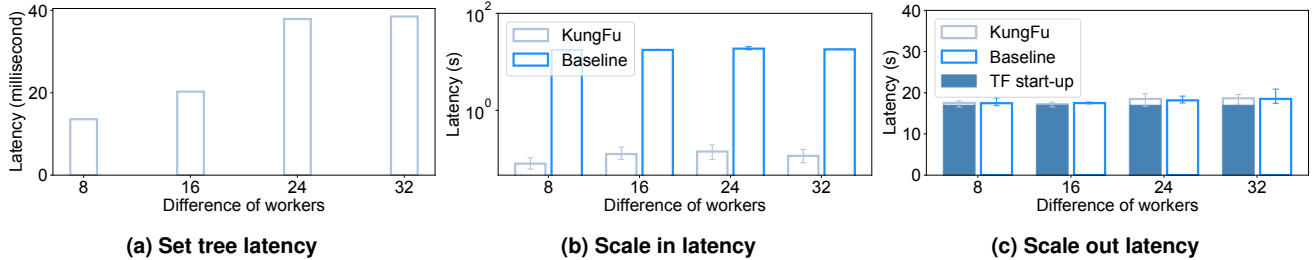
Fig. 7: Adaptation overhead
