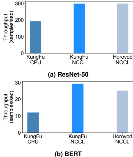
Fig. 10: Training throughput
