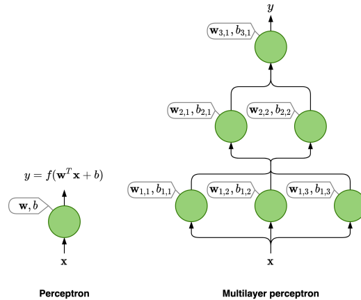
(b) Perceptron and multilayer perceptron, f(\cdot) is an activation function.
