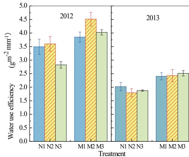
Fig. 4 - The summer maize WUE during 2012 and 2013 summer maize growing seasons. Codes represent 10.0 plants \text{m}^{-2} density without straw mulching (N1), 10.0 plants \text{m}^{-2} density with 0.6 \text{kg m}^{-2} straw mulching (M1), 7.5 plants \text{m}^{-2} density without straw mulching (N2), 7.5 plants \text{m}^{-2} density with 0.6 \text{kg m}^{-2} straw mulching (M2), 5.5 plants \text{m}^{-2} density without straw mulching (N3), and 5.5 plants \text{m}^{-2} density with 0.6 \text{kg m}^{-2} straw mulching (M3), respectively
