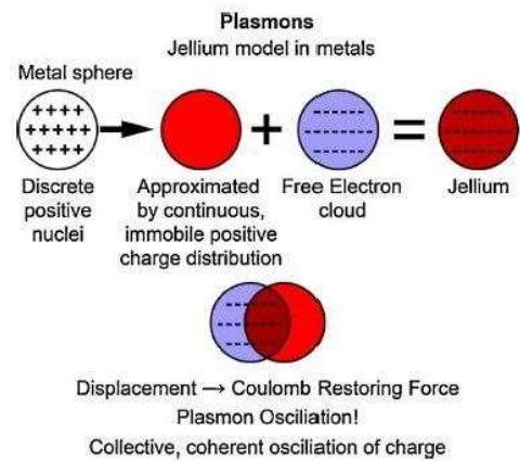
Figure 10: Plasmon [22]
