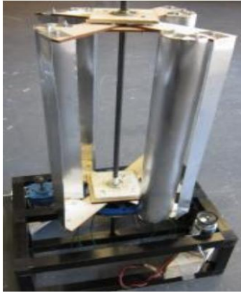
Figure 1: Vertical Axis Wind Turbine- Savonius type [1]
