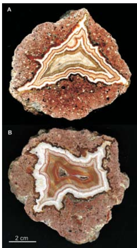
Fig. 1. Multi-coloured volcanic agates from Novy Kościół (Poland) with typical fortification banding
