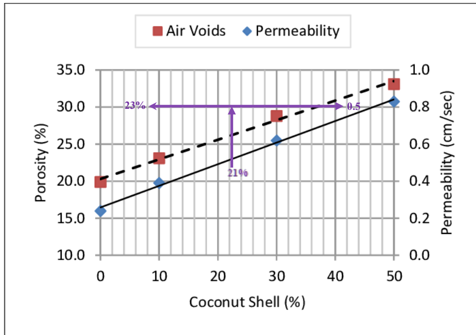
FIGURE 4. Permeability and porosity result.
