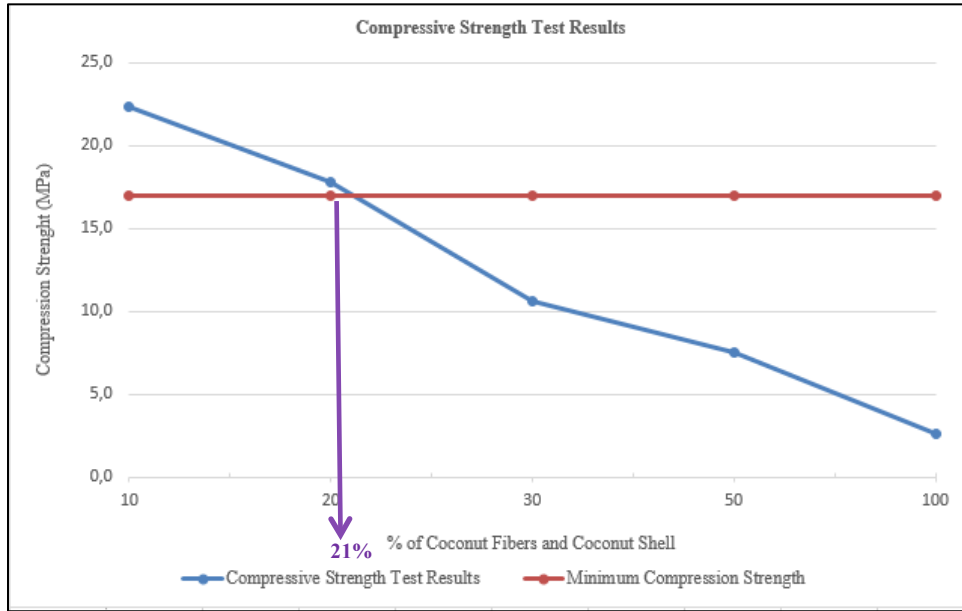
FIGURE 3. Compressive strength test result.
