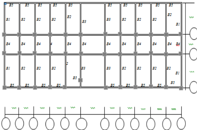
Fig 1.: The Floor Beam System
