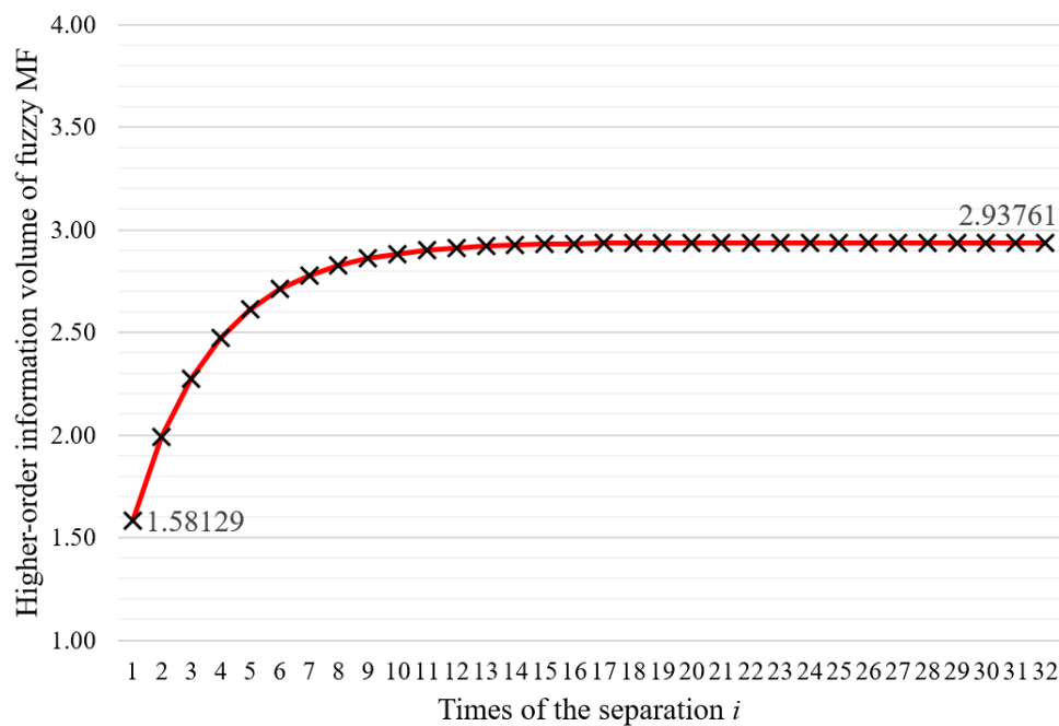
Figure 2: The convergence tendency of H_\infty(\mu, v) in Example 4.3
