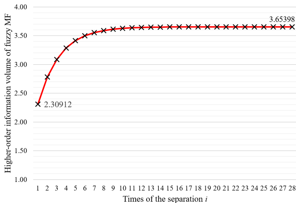
Figure 3: The convergence tendency of H_\infty(\mu, v) in Example 4.4
