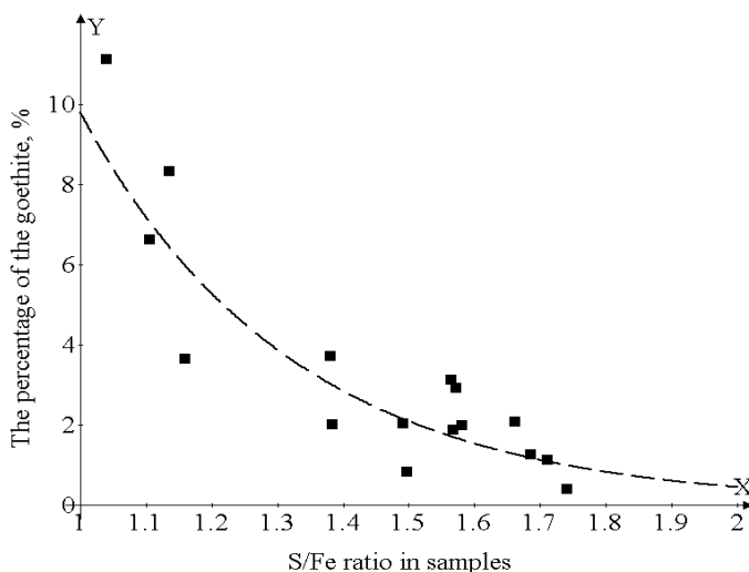
Fig. 2. Dependence of goethite percentage on S/Fe ratio in samples
