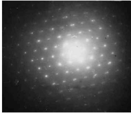
Fig. 3 Reciprocal lattice received with the method of electronic diffraction of troilite sputtered to the glass surface
