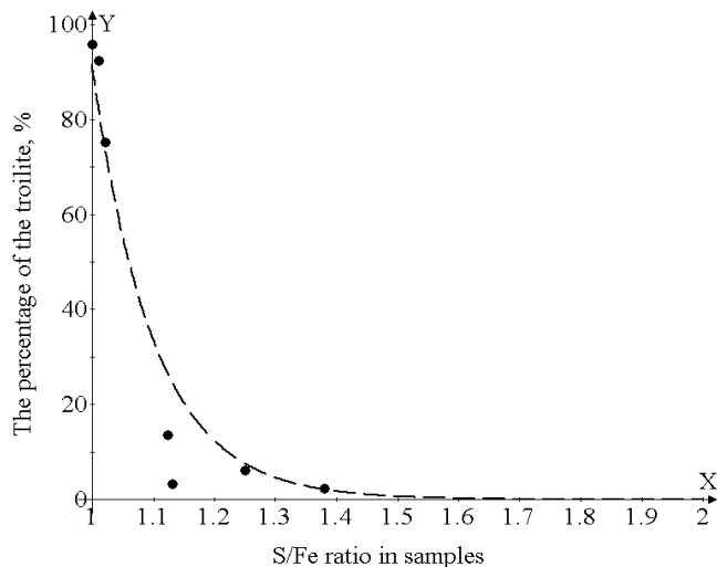
Fig. 1. Dependence of troilite percentage on the sulphur and iron ( S/Fe ) ratio in samples
