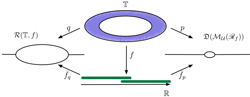
Fig. 5 An example of the enhanced mapper graph \mathfrak{D}(\mathcal{M}_{\mathcal{U}}(\mathcal{R}_f)) and the Reeb graph \mathcal{R}(\mathbb{T}, f) of the height function f on the torus \mathbb{T} , with an open cover \mathcal{U} of f(\mathbb{T}) consisting of two open intervals. The maps q and \bar{f}_q are the natural quotient factorization of f obtained from the definition of the Reeb graph. Similarly, p and \bar{f}_p are the quotient map and factorization of f obtained from the definition of the enhanced mapper graph
