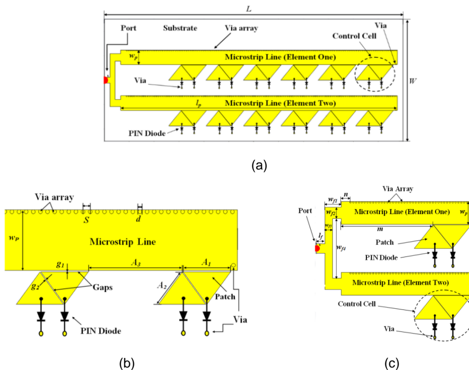
Figure 1. Reconfigurable HW-MLWAs array: (a) top view, (b) microstrip line with control cell, (c) port and feed line for two elements.
