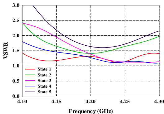
Figure 6. VSWA for the HW-MLWA array for the switches configuration for all cases in for the switches configuration for all cases Table 2
