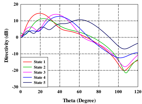
Figure 5. Radiation patterns of the proposed antenna at 4.2GHz for different switch cases in Table 1
