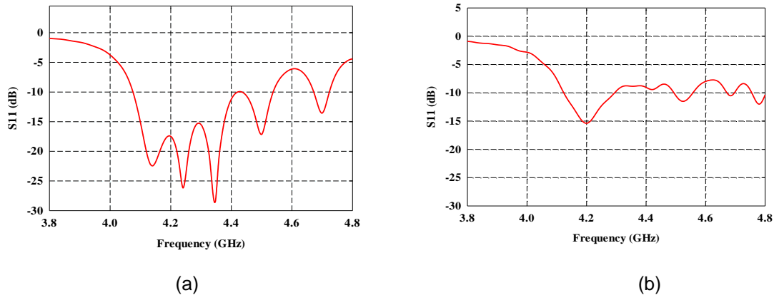
Figure 2. |S_{11}| for the (a) state 1 and (b) state 2 of the proposed antenna
