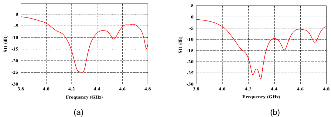
Figure 3. |S_{11}| for the (a) state 3 and (b) state 4 of the proposed antenna
