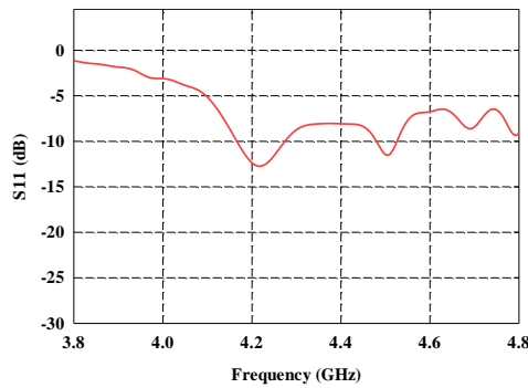
Figure 4. |S11| for the state 5 of the proposed antenna
