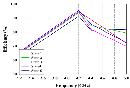
Figure 7. Efficiency for the HW-MLWA array for the switches configuration for all cases in Table1
