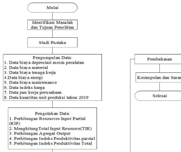
Gambar 1. Flowchart Penelitian
