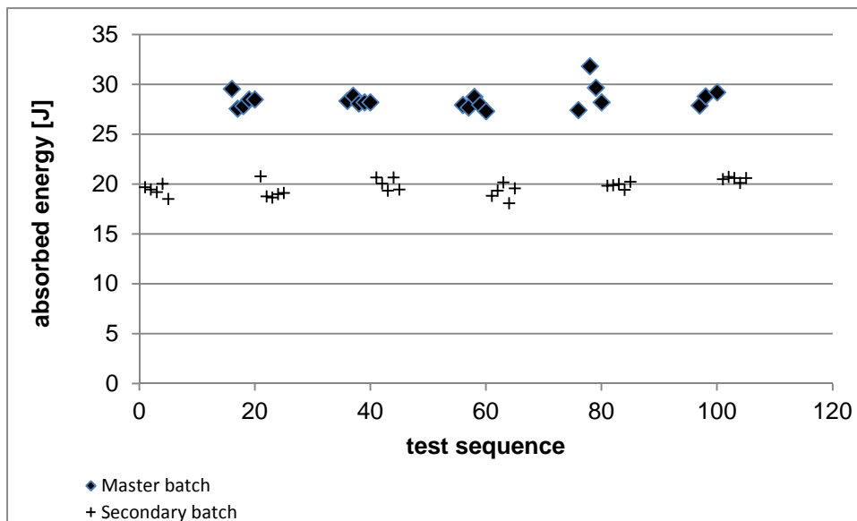
Figure 3: Absorbed energy values of 22 test pieces of ERM ® -FA013ba, compared with 30 test pieces of ERM ® -FA013bu; data are displayed in the actual test sequence
