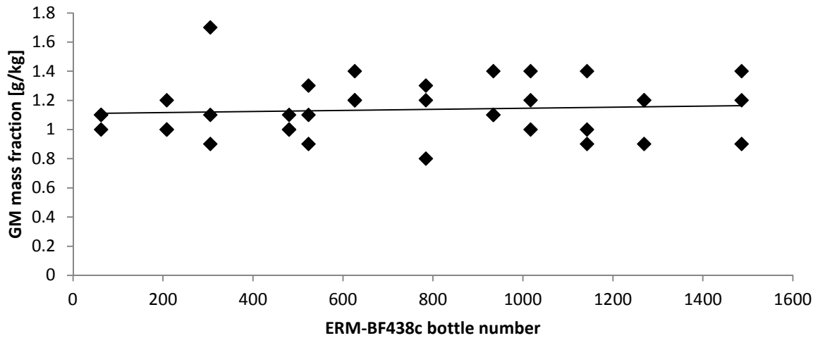
Figure B1: Real-time PCR measurement results obtained for ERM-BF438c. Three samples (extraction replicates) were measured from each of 12 randomly selected bottles ( N = 12 , n = 3 ), with each sample measured in 3 real-time PCR replicates. The straight line is a least-squares linear regression through all data points.
