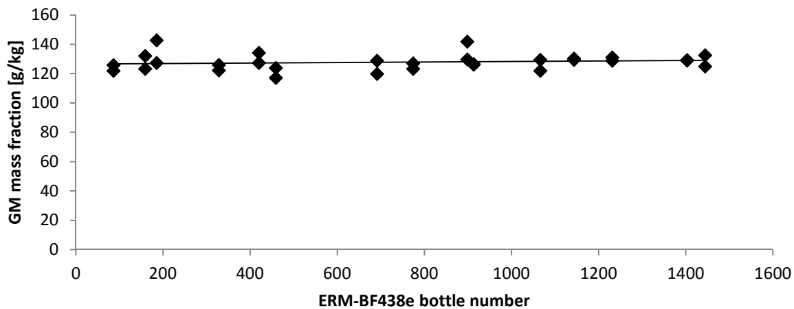
Figure B3: Real-time PCR measurement results obtained for ERM-BF438e after analytical trend correction. Two samples (extraction replicates) were measured from each of 15 randomly selected bottles ( N = 15 , n = 2 ), with each sample measured in 3 real-time PCR replicates. The straight line is a least-squares linear regression through all data points.
