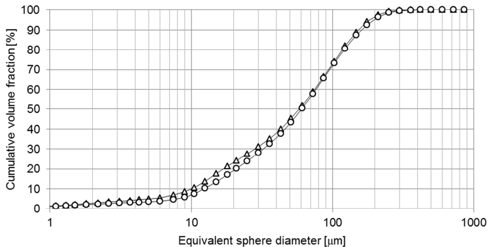
Figure 1: Cumulative distribution of particle volume fractions in the GM powder ( \circ ) and non-GM powder ( \Delta ) analysed by laser diffraction ( N = 1, n = 3 ). The total particle volume for each material is set as 100 %.
