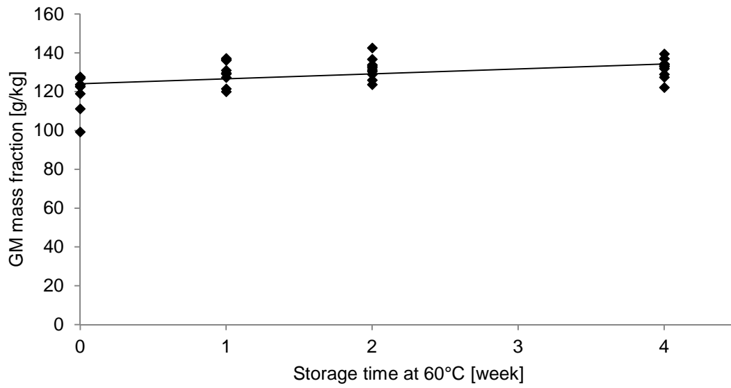
Figure C3: Real-time PCR measurement results obtained for ERM-BF438e during short-term stability testing at 60 °C. For each storage time, 2 samples (extraction replicates) were measured from each of 5 randomly selected bottles ( N = 5 , n = 2 ), with each sample measured in 3 real-time PCR replicates. The straight line is a least-squares linear regression through all data points.
