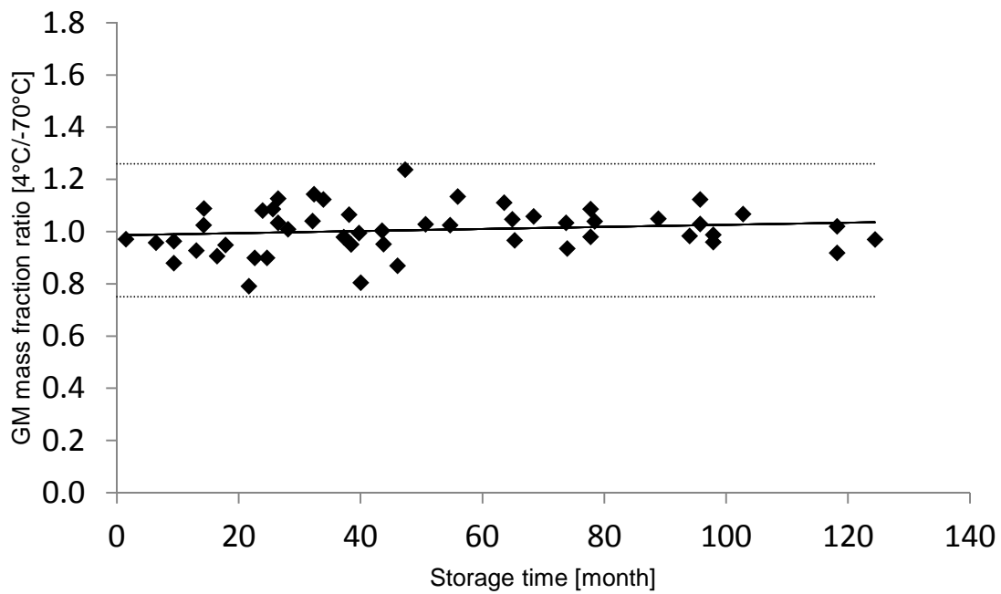
Figure D1: Real-time PCR measurement results obtained for ERM-BF411, ERM-BF412, ERM-BF413, ERM-BF413k, ERM-BF414, ERM-BF415, ERM-BF416, ERM-BF417, ERM-BF418, ERM-BF420, ERM-BF424, ERM-BF427 and ERM-BF433 during post-certification monitoring. The dashed lines give the limits of 3 s obtained for the measurement results. The straight line is a least-squares linear regression through all data points.
