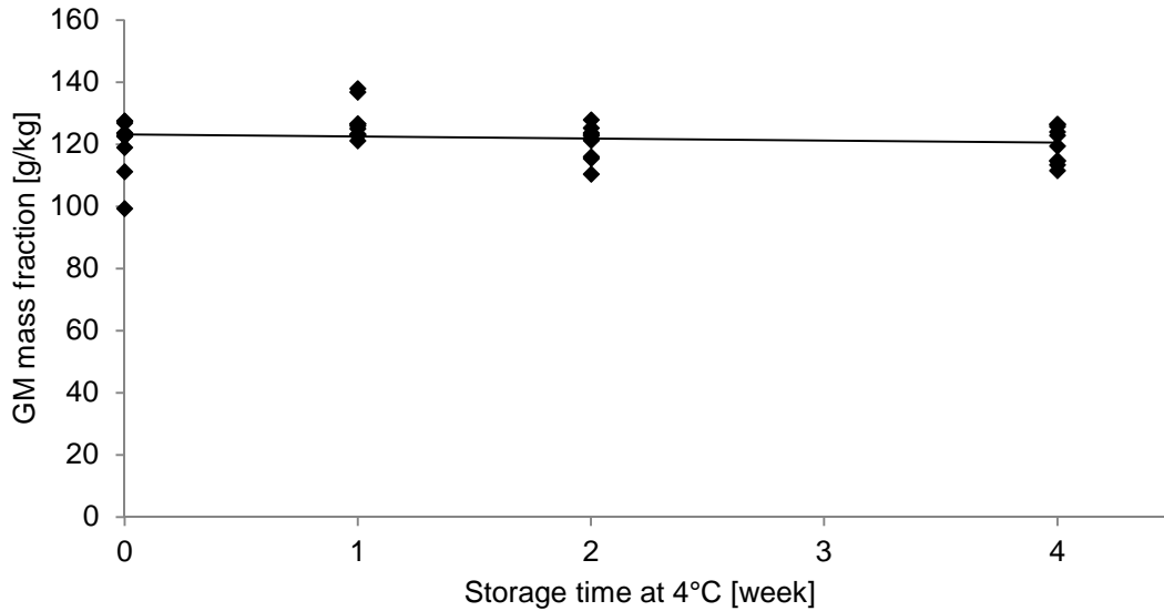
Figure C1: Real-time PCR measurement results obtained for ERM-BF438e during short-term stability testing at 4 °C. For each storage time, 2 samples (extraction replicates) were measured from each of 5 randomly selected bottles ( N = 5 , n = 2 ), with each sample measured in 3 real-time PCR replicates. The straight line is a least-squares linear regression through all data points.
