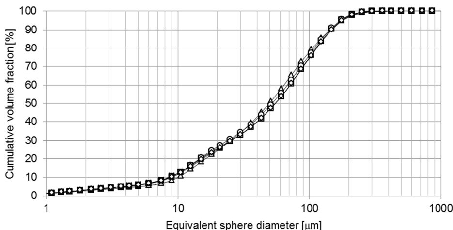
Figure 2: Cumulative distribution of particle volume fractions in ERM-BF438a (x), ERM-BF438b ( \Delta ), ERM-BF438c ( \square ), ERM-BF438d ( \circ ) and ERM-BF438e ( \diamond ) analysed by laser diffraction ( N = 5 , n = 2 ). The total particle volume for each preparation is set as 100 %.
