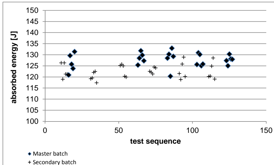
Figure 3: Absorbed energy values of 25 test pieces of ERM ® -FA016ax, compared with 30 test pieces of ERM ® -FA016bj; data are displayed in the actual test sequence
